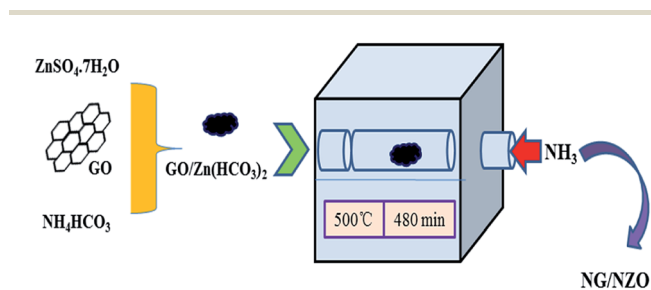
Scheme 1 Schematic preparation of NG/NZO nanocomposites.
