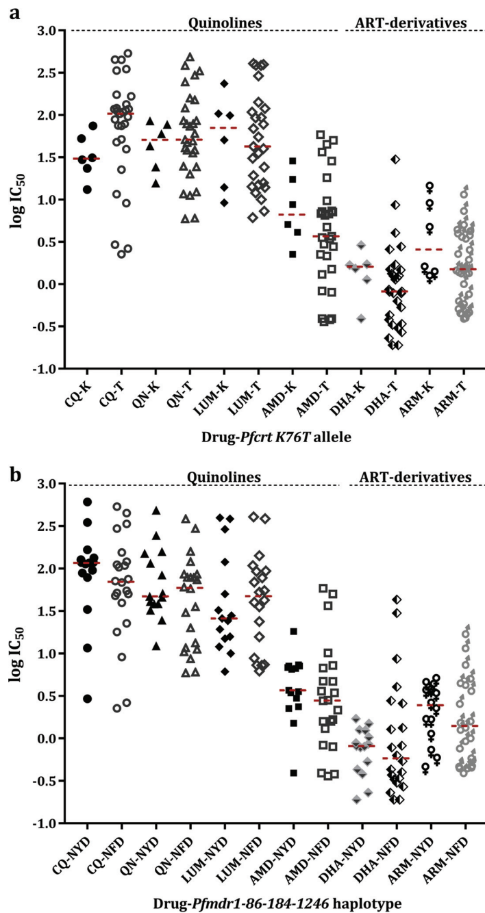
FIG 5 In vitro sensitivity ( IC_{50} ) of Plasmodium falciparum isolates collected in the year 2015 for mutant or wild-type alleles at pfprt K76T codon (a) and pfmdr1-86-184-1246 haplotypes of isolates assayed against quinolines (CQ, QN, LUM, and AMD) and artemisinin derivatives (DHA and ARM) (b). Each point in a group represents the \log IC_{50} for an isolate with the specific allele or haplotype and drug labeled on the x axes. Broken red lines show the median \log IC_{50} values for each haplotype group per drug.
