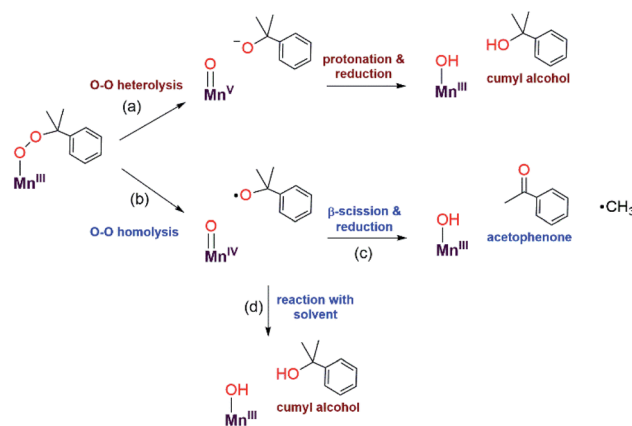
Scheme 2 Possible decay pathways for [\text{Mn}^{\text{III}}(\text{OOCm})(^{\text{6Me}}\text{dpaq})](\text{OTf}) .
