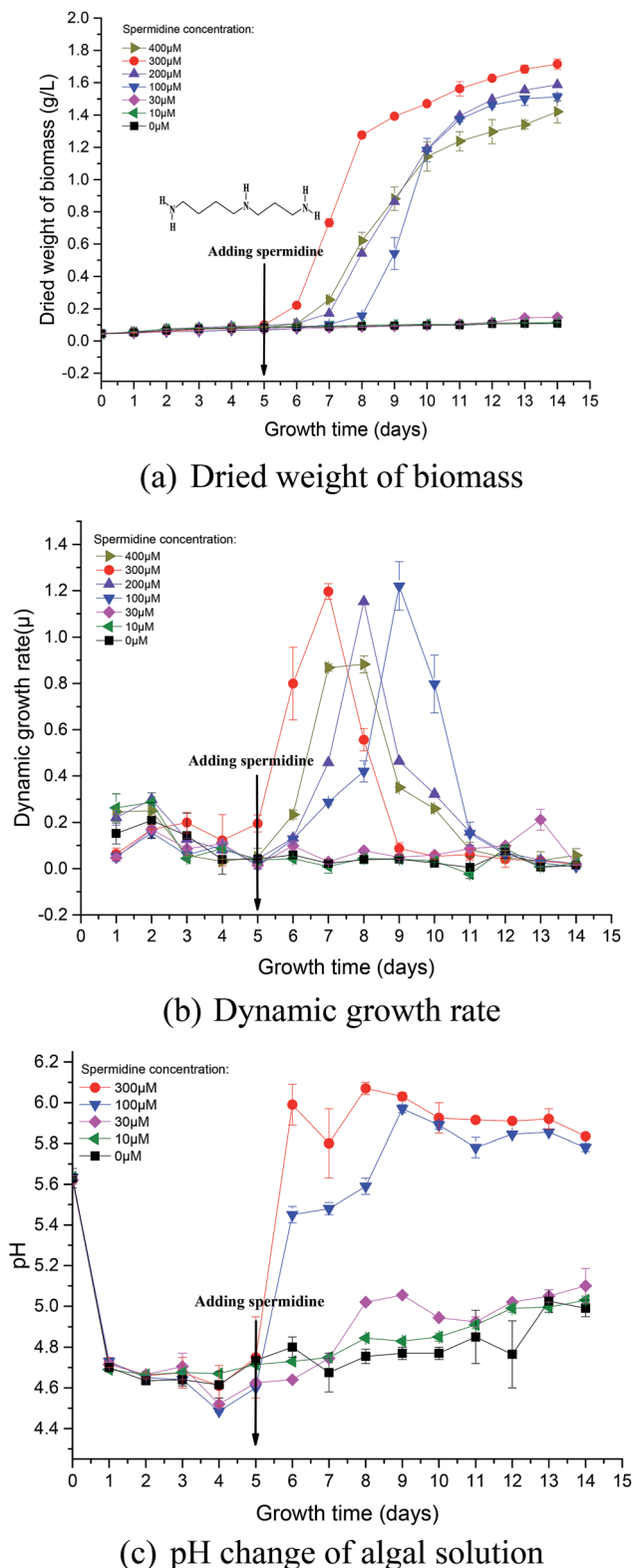
Fig. 1 Growth curves (a and b) and pH change (c) of Chlorella under a high CO 2 concentration (15%) and high light intensity (30 000 lux).
