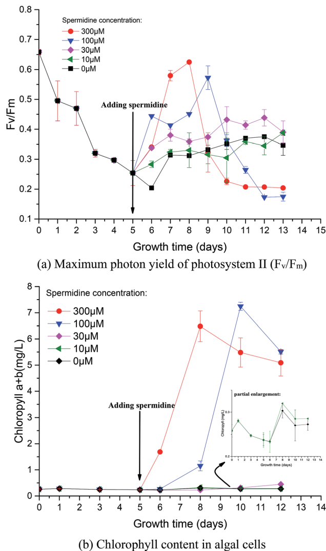
Fig. 2 Photosynthesis (a) and chlorophyll synthesis (b) of Chlorella under a high CO 2 concentration (15%) and high light intensity (30 000 lux).
