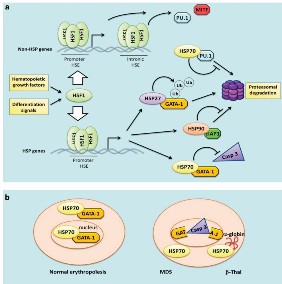
Figure 1 Mechanisms of action of HSF and HSPs in the control of expression and stability of hematopoietic transcription factors. (a) Upon differentiation signals, HSF1 gets activated, trimerized, and binds HSE elements found in either the promoter or intronic regions of HSPs and non-HSPs genes. Critical transcription factors are then protected from caspase-3 cleavage (Casp 3), from proteasomal degradation, or conversely oriented towards proteolysis depending on the stage of differentiation and the needs of the cell. (b) In contrast to normal erythropoiesis, HSP70 cannot be translocated into the nucleus of erythroid progenitors from MDS and from beta-thalassemia major ( \beta -Thal) patients. GATA-1 is no more protected and subsequently cleaved by caspase-3
