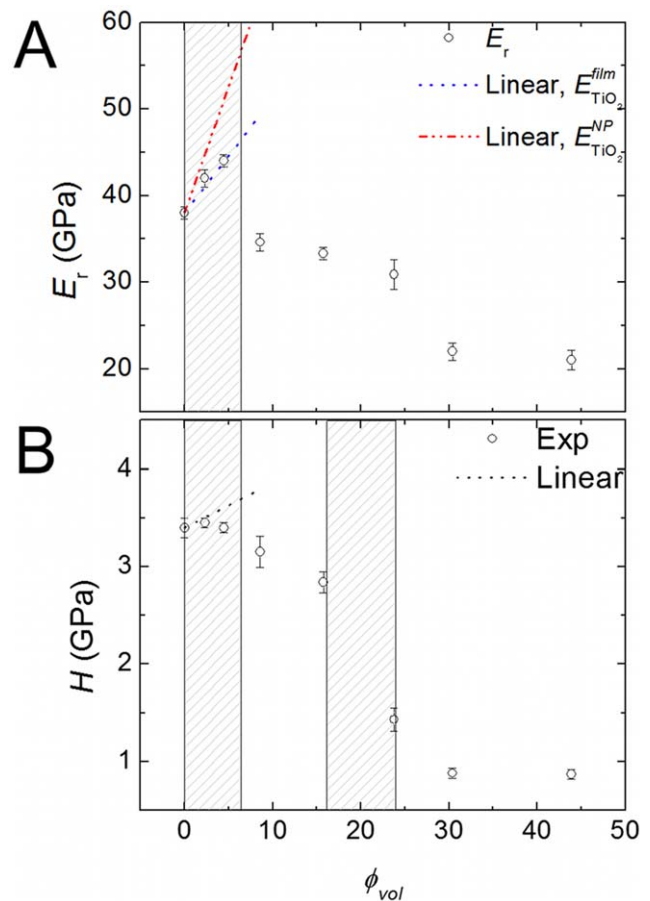
Figure 3. Variation of the mechanical properties with the composition of the hybrids. (A) Effective reduced Young's modulus, E_r , of hybrids with increasing TiO 2 content, \phi_{TiO_2} . The symbols correspond to the experimental values and the error bars to the standard deviation from several indentations (see text). The dotted and dash-dotted lines correspond to a linear variation of E_r from the rule of mixtures (see text) using E_{TiO_2}^{film} \approx 170 GPa [53,54] or E_{TiO_2}^{NP} \approx 330 GPa, [45] respectively; and E_{NFC} = 38 GPa (this work). The hatched region indicates the region where the linear increase is observed. (B) Variations of hardness, H , as a function of \phi_{TiO_2} . The dotted line in (b) corresponds to a linear variation of H (see text) assuming H_{TiO_2} \approx 10 GPa [53,54] and H_{NFC} = 3.4 GPa (this work). The hatched regions represent the areas of high hardness and the transition region toward low hardness. doi:10.1371/journal.pone.0045828.g003
