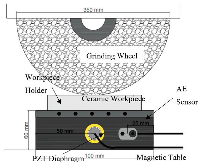
Figure 2. Experimental setup.
