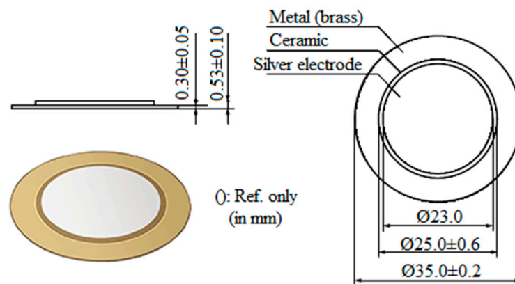
Figure 1. Murata piezoelectric sensor 7BB-35-3 used in the tests.
