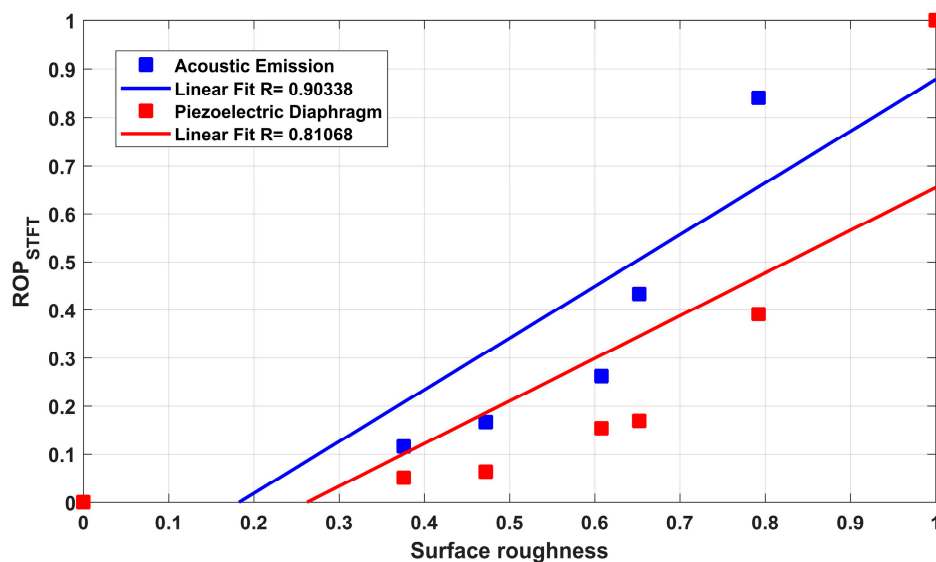
Figure 7. Correlation between ROP and surface roughness for both sensors.
