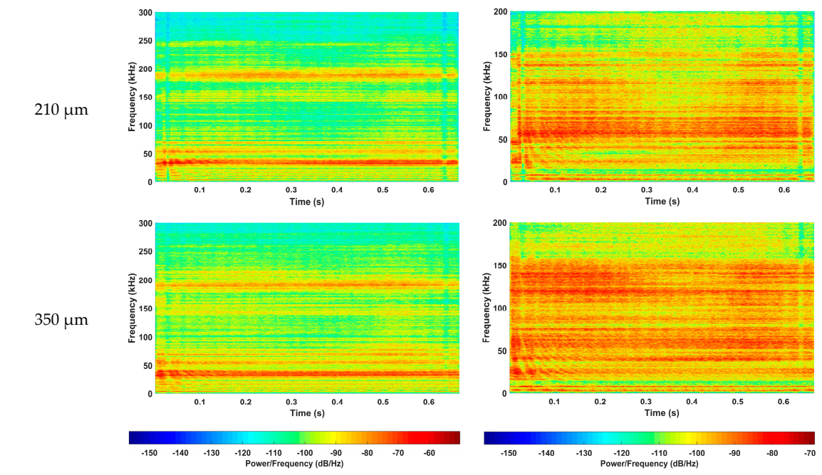
Figure 4. Short-time Fourier transform (STFT) spectrograms.
