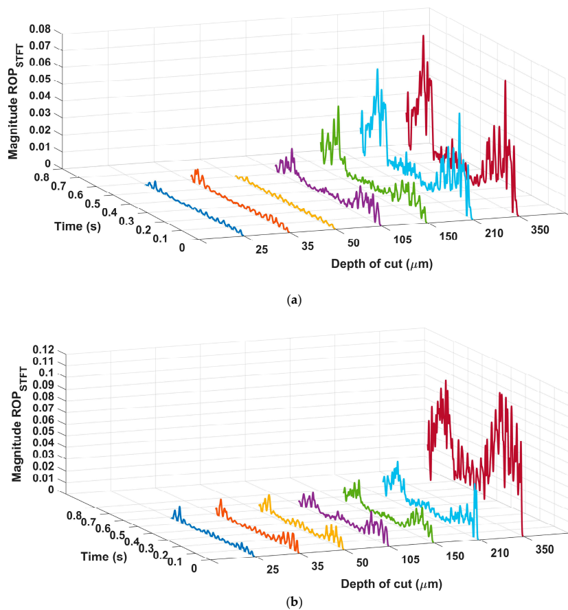
Figure 5. The ratio of power (ROP) of the (a) acoustic emission sensor (AE) and (b) piezoelectric diaphragm (PZT).
