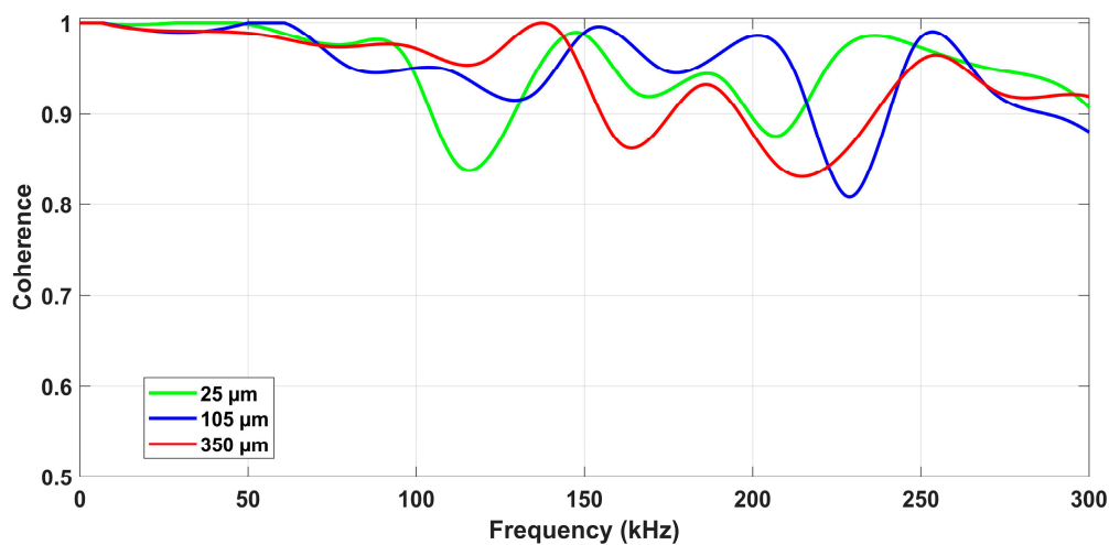
Figure 6. Magnitude-squared coherence between the AE sensor and PZT diaphragm at three grinding conditions.
