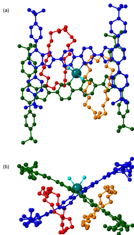
Fig. 6 Single-crystal-X-ray structure of the complex formed from a solution with a 1 : 1 Zn to 4 ratio; [\text{Zn}(4)_2(\text{DMF})(\text{H}_2\text{O})](\text{NTf}_2)_2 . (a) Side view emphasizing the octahedral coordination geometry at \text{Zn}(\text{II}) . (b) Top view showing the relative positions of the crown ether macrocycles on the rotaxane ligands. Rotaxanes are coloured blue axle with red wheel and green axle with orange wheel. Only the O-atoms of the coordinated DMF and water molecules are shown for clarity. Anions are not shown. All H-atoms are omitted for clarity.
