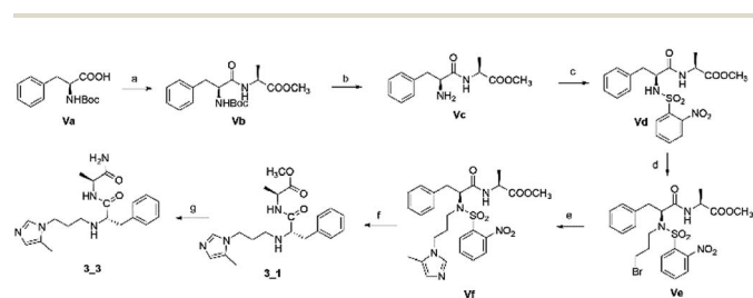
Scheme 2 Synthetic route for 3_x series compounds. Conditions and reagents: (a) L-alanine methyl ester hydrochloride, HOBt, EDC, TEA, MeCN, r.t., 12 h; (b) TFA, TIPS, DMC, r.t., o.n.; (c) 2-nitrobenzenesulfonyl chloride, TEA, DMC, 0 °C to r.t., 4 h; (d) 1,3-dibromopropane, Cs 2 CO 3 , DMF, 60 °C, 6 h; (e) 5-methyl-1-trityl-1 H -imidazole, MeCN, reflux, 24 h then MeOH, THF, reflux, o.n.; (f) thiophenol, K 2 CO 3 , MeCN, r.t., o.n.; (g) NH 3 , MeOH, r.t., o.n.
