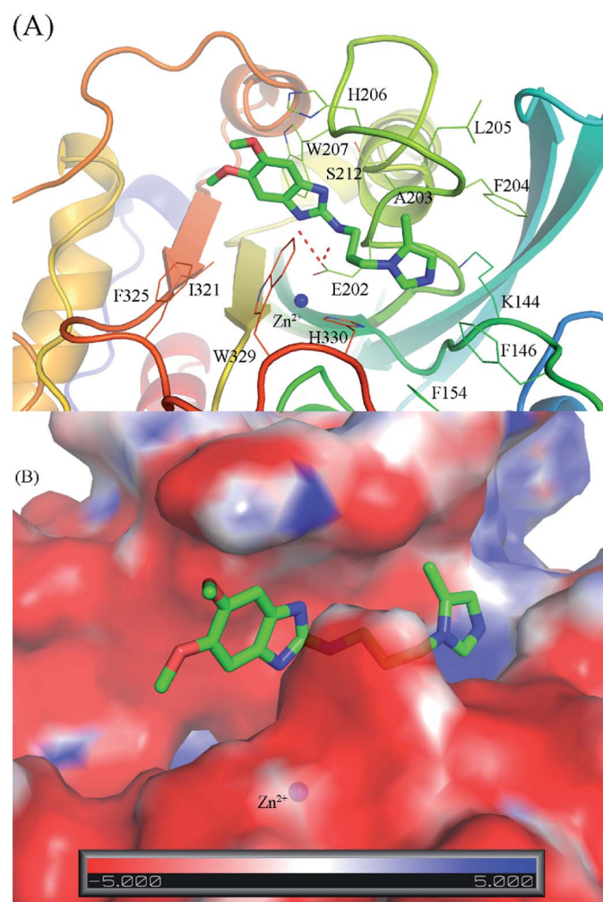
Fig. 5 The binding pose of compound 1_2 with the hQC enzyme obtained over 50 ns of MD simulations. (A) The critical residues of hQC form sidechain and hydrogen bond contacts with compound 1_2; (B) the charged surface of the hQC enzyme in the binding mode with compound 1_2.
