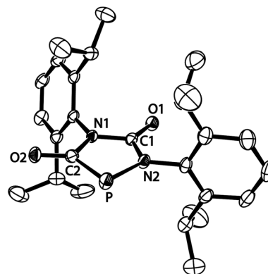
Fig. 2 ORTEP plot of [4a] - (thermal ellipsoids are drawn at 50% probability). Hydrogen atoms have been omitted for clarity. Selected bond lengths (Å) and angles (°): C1–N1 1.378(3), N1–C2 1.425(3), C2–P 1.756(3), C2–O2 1.254(3), P–N2 1.779(2), N2–C1 1.347(3), C1–O1 1.245(3); C1–N1–C2 115.9(2), N1–C2–P 110.0(2), C2–P–N2 88.3(1), P–N2–C1 115.8(2), N2–C1–N1 110.1(2).
