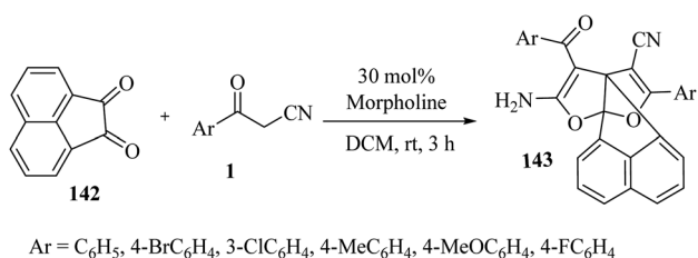
Scheme 55 Synthesis of fused (epoxyetheno)indeno-furans 143 .
