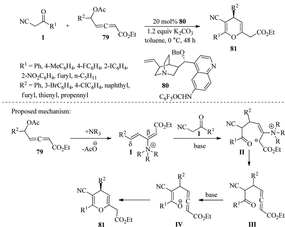
Scheme 31 Synthesis of 4H-pyrans 81 by using 6'-deoxy-6' perfluorobenzamido-quinine 80 as a catalyst.
