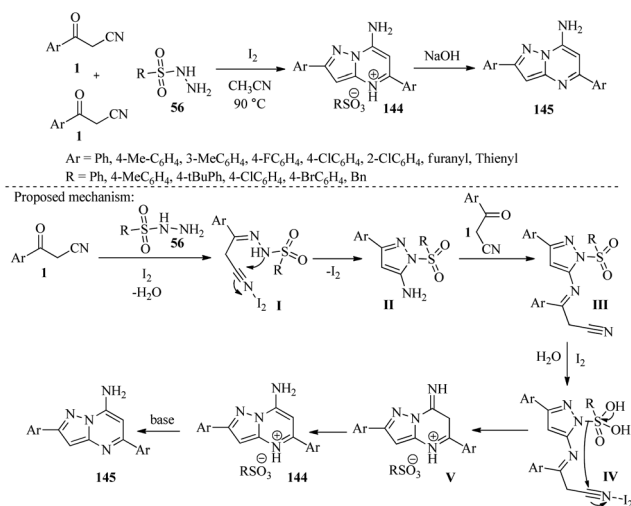
Scheme 56 Synthesis of functionalized pyrazolo[1,5- a ]pyrimidine-4-ione sulfonates 144 and pyrazolo[1,5- a ]pyrimidines 145 .
