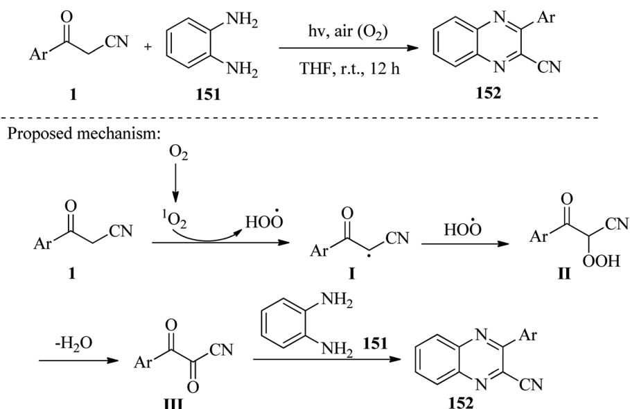
Scheme 59 Synthesis of quinoxaline derivatives 152 .
