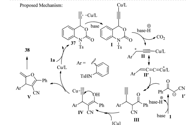
Scheme 16 Synthesis of tetrasubstituted furan 38 .
