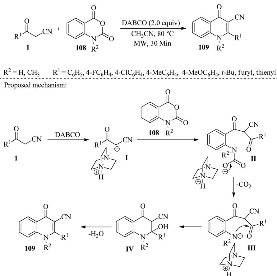
Scheme 41 Synthesis of 3-cyano-4-quinolone derivatives 109 .
