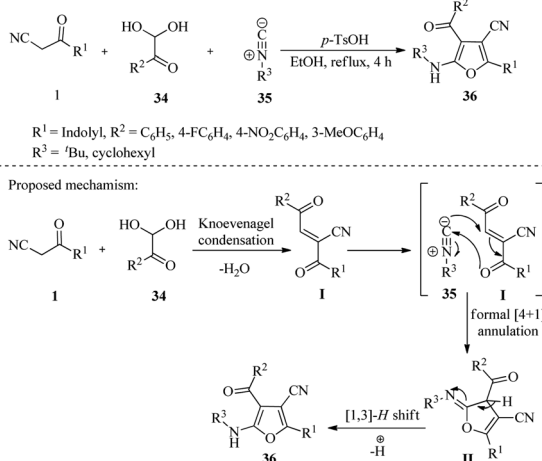
Scheme 15 Synthesis of highly substituted furan-linked biheteroaryls 36 .
