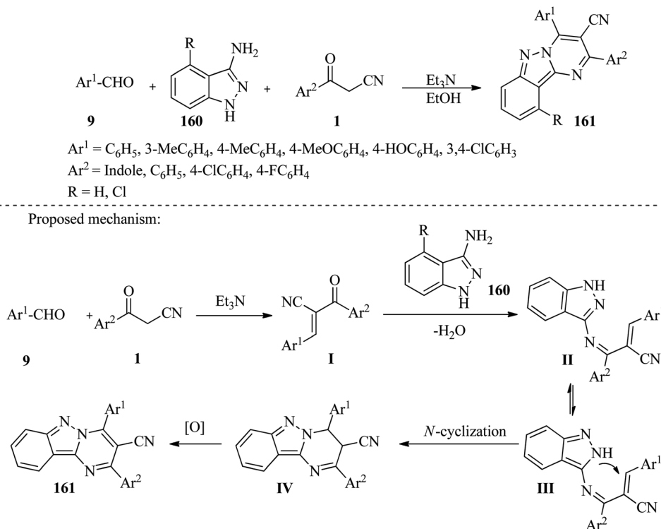
Scheme 62 Synthesis of pyrimido[1,2- b ]indazol-3-carbonitrile derivatives 161 .
