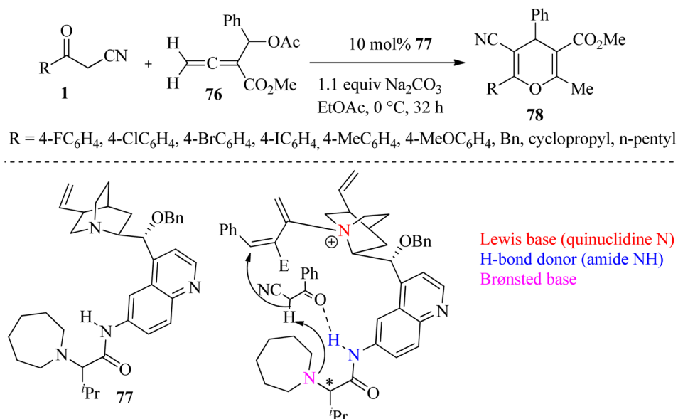
Scheme 30 Synthesis of 4H-pyran derivatives 78 by using 6'-deoxy-6'-(1-( N,N -(2,2'-oxydiethyl)-valine amido)quinine 77 as a catalyst.
