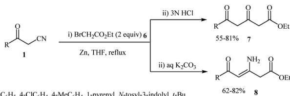
Scheme 3 Synthesis of 3,5-dioxopentanoates 7 (3,5-diketo esters) and 3-amino-5-oxopent-3-enoates 8 .
