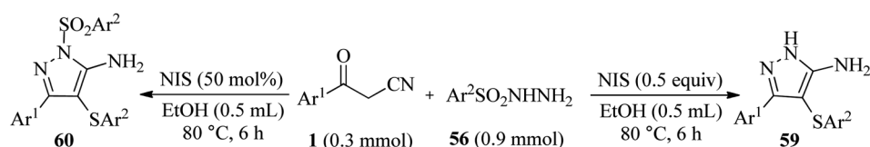
Scheme 23 Synthesis of 3-aryl-4-(arylthio)-1 H -pyrazol-5-amine derivatives 59 and 3-phenyl-1-(phenylsulfonyl)-4-(phenylthio)-1 H -pyrazol-5-amines 60 .
