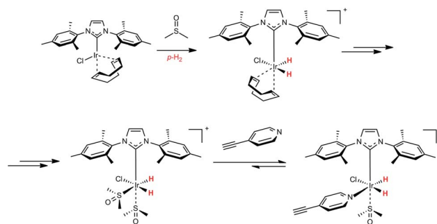
Scheme 2 A basic scenario of the activation of the Ir-Mes pre-catalyst with DMSO, and the consecutive reaction of the activated Ir complex with 1 .
