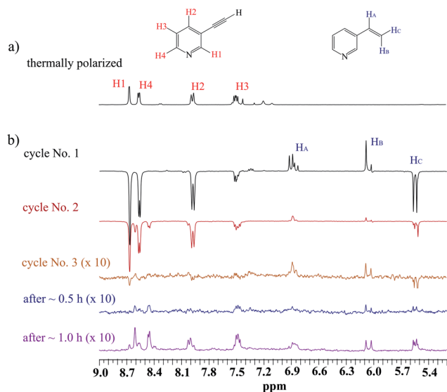
Fig. 1 The ^1\text{H} NMR spectra of the mixture of 1 with the 10 mol% Ir-Mes pre-catalyst in MeOD- d_4 at 298 K; (a) before p\text{-H}_2 administration (b) several consecutive hyperpolarization experiments.
