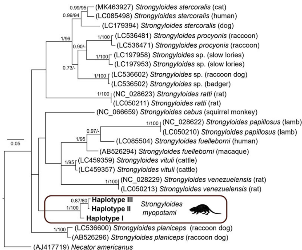
Figure 6. Phylogenetic tree of 25 sequences of Strongyloides species reconstructed by Bayesian inference. The tree is rooted using Necator americanus as an out-group. Values at the nodes indicate posterior probabilities from BI and bootstrap values from ML analyses. Dashes indicate nodal support values below 0.70 and 50, respectively. The hosts of respective Strongyloides specimens are noted in brackets.
