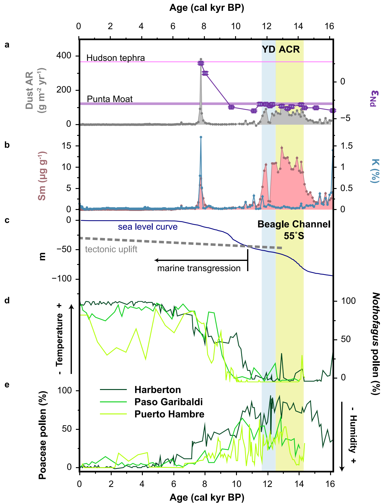
Figure 2. Paleoenvironmental data from the Southern Hemisphere. a , Dust accumulation rate ( \text{g m}^{-2} \text{yr}^{-1} ) and neodymium isotopic composition ( \epsilon_{\text{Nd}} ) of the inorganic fraction of peat samples at the Harberton bog ( 54.9^{\circ}\text{S} , 67.2^{\circ}\text{W} ; this study). b , Sm ( \mu\text{g g}^{-1} ) and K (%) concentrations in bulk peat samples from Harberton bog (this study). c , Estimated eustatic sea level curve and local tectonic uplift (m) of the Beagle Channel area 19 . d,e , Nothofagus and Poaceae pollen records (%) from Harberton 58 , Paso Garibaldi 4 and Puerto Hambre 20 bogs (Tierra del Fuego and South-Patagonia). ACR = Antarctic Cold Reversal; YD = Younger Dryas.
