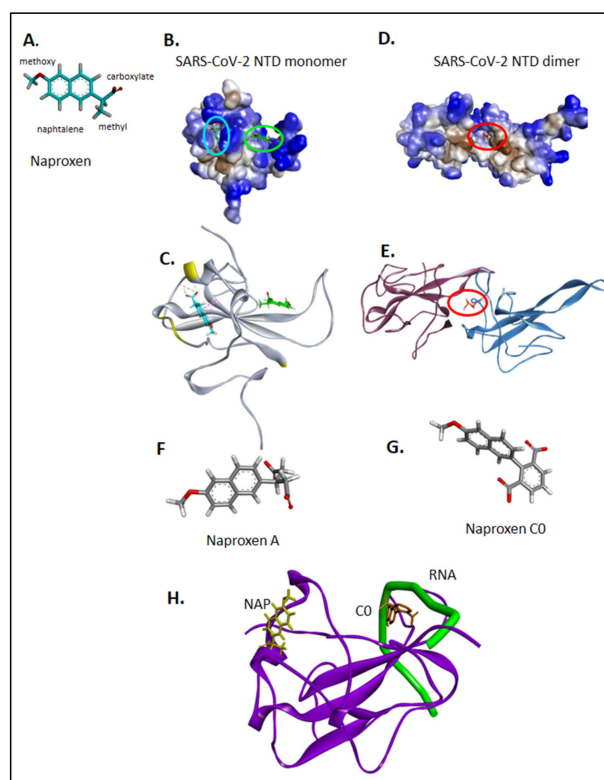
Figure 2. Binding sites of naproxen to N NTD monomer and dimer; comparison with naproxen derivatives. Naproxen is shown in (A), with details on its functional moieties as discussed in the text. Panels (B,C) show the binding sites of naproxen on monomeric N NTD (PDB 7ACT) [28], the main (more frequent) binding site represented in cyan, is associated with the dimeric interface, highlighted in (C) in yellow; the minor site of naproxen on monomeric N NTD is represented in green. In panels (D,E) is shown the main binding site of naproxen on dimeric N NTD (PDB 6VYO) [27]. For details, see also Supplementary Figure S2. The structures of naproxen A and C0 are shown in panels (F) and (G), respectively. Panel (H) summarizes the RNA binding site (shown in green) deduced from RMN studies [28], the main binding site of naproxen on the left and the main binding site of naproxen C0, located within the RNA binding groove. (See also Table 1 and Supplementary Figure S2).
