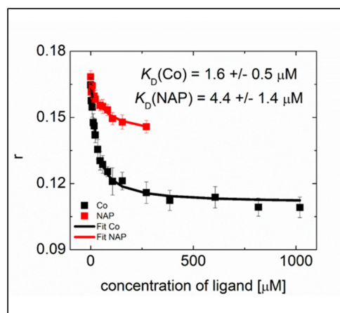
Figure 4. Competition on N NTD of binding of RNA with naproxen or naproxen C0 deduced from fluorescence anisotropy r .
