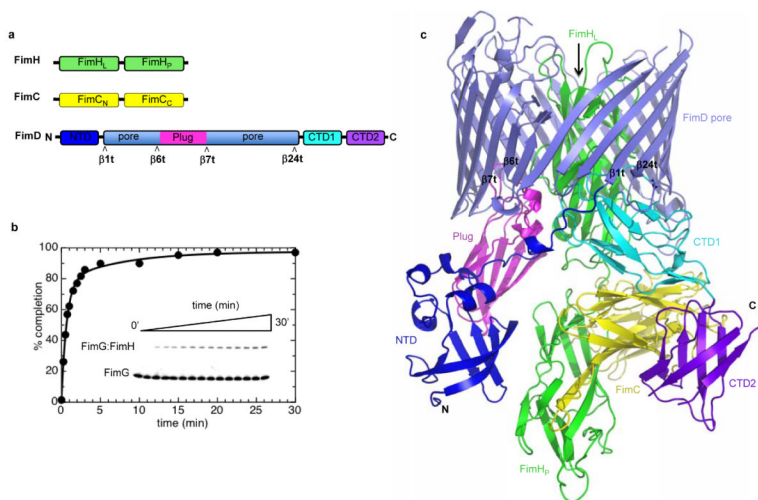
Fig. 1. Structure of the FimD:FimC:FimH complex
