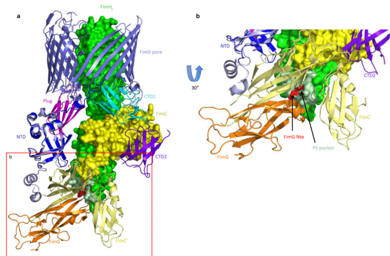
Fig. 4. Chaperone:subunit incorporation cycle at the FimD usher
