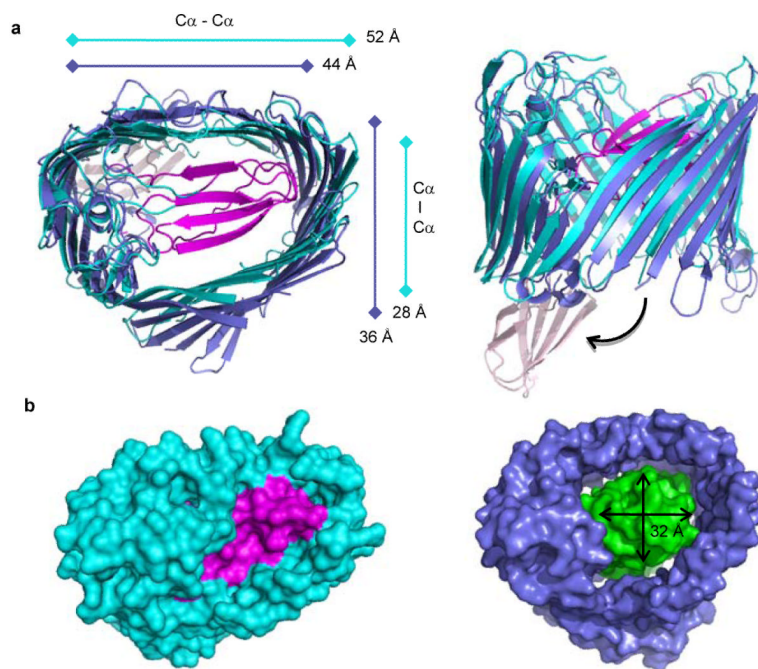
Fig. 2. Channel conformations in apo and activated (FimC:FimH-engaged) FimD usher a , top ( left ) and side ( right ) view ribbon representations of the superimposed apo-FimD (cyan) and activated FimD (slate) \beta -barrel. The plug domain in the channel lumen in apo FimD (magenta) rotates into the periplasm following FimD activation (pink). b , top view surface representation of the apo-FimD ( left ) and activated FimD ( right , for clarity, showing only the translocation channel and FimH lectin domain, FimH L ). The plug and FimH L are coloured magenta and green, respectively.
