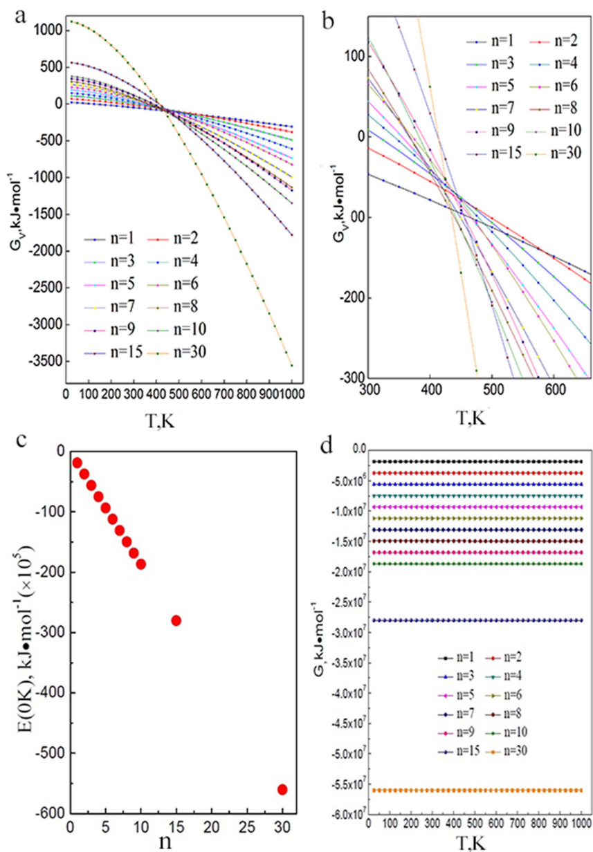
Figure 1 | The thermodynamic properties of (\text{Al}_2\text{O}_3)_n with n = 1-10, 15 and 30 at 0-1000 K. (a) The values of the vibrational free energy, G_v , of (\text{Al}_2\text{O}_3)_n are plotted as a group of colored solid curves. (b) A magnified section of (a) in the region of the intersection of the G_v values of (\text{Al}_2\text{O}_3)_n . The temperature range of the region of the intersection is approximately 350 K to 600 K. (c) The zero-point energy at a temperature of 0 K, E(0\text{K}) . (d) The Gibbs free energy, G , where G = G_v + E(0\text{K}) .
