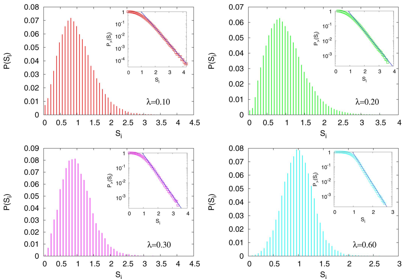
Figure 4 | Distribution of the node strengths. In the plots we report the distribution of the outgoing strength of the nodes, P(S_i) , for T = 100 and \lambda = 0.1, 0.2, 0.3, 0.6 . Notice that for all \lambda values the distributions P(S_i) are homogeneously distributed around the corresponding mean values \langle S_i \rangle . The insets of each plot report the cumulative distributions, P_{>}(S_i) = \sum_{x \geq S_i} P(x) , to show the exponential decay of the tails of P(S_i) .
