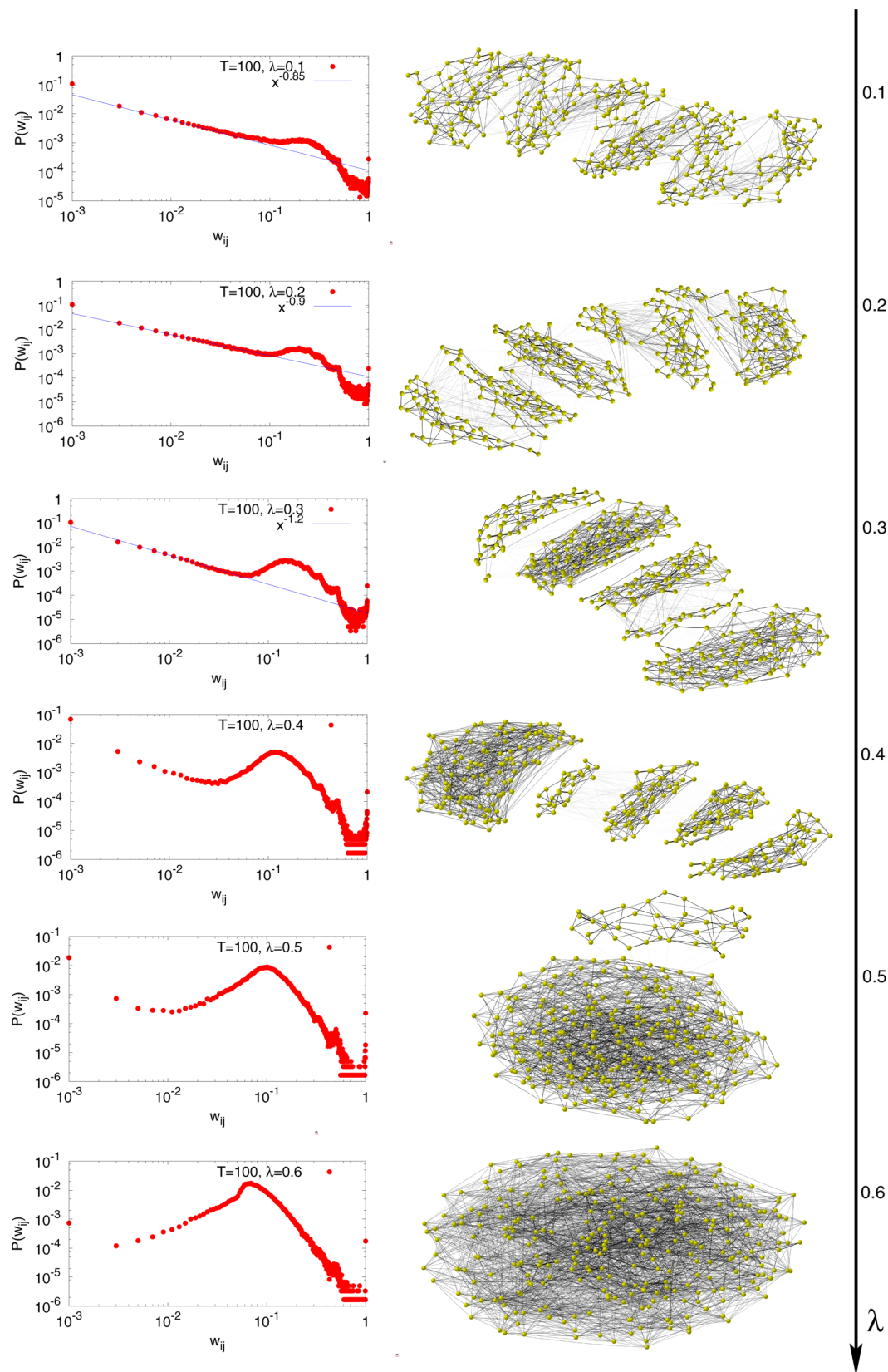
Figure 3 | Network structure, and corresponding distribution of the link weights. In the left panels we report the distribution of the weights, P(W_{ij}) , for the case T = 100 , and for different values of \lambda (increasing from \lambda = 0.1 to \lambda = 0.6 ). Notice that the regime of small \lambda ( \lambda = 0.1 , \lambda = 0.2 and \lambda = 0.3 ) displays a power law distribution of weights, P(W_{ij}) = W_{ij}^{-\alpha} . In the right part of the panels we show different snapshots of the network structure for the corresponding values of \lambda . Note that as \lambda increases from \lambda = 0.1 to \lambda = 0.4 the modules increase in size and tend to be less overlapping until the network breaks up into several unconnected components.
