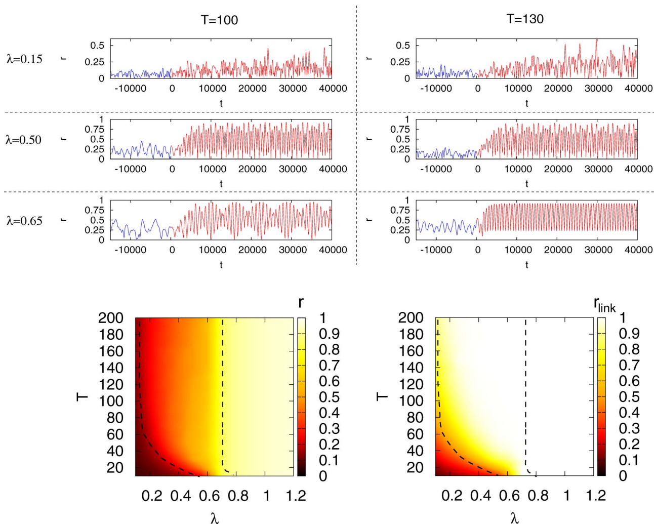
Figure 1 | Time evolution of the global order parameter and phase diagrams. In the top panels the time evolution of the Kuramoto order parameter r is reported for T = 100, 130 and \lambda = 0.15, 0.50, 0.65 . The dynamics of the oscillators is initially implemented on a fixed network, while for t > 0 the weights evolve according to equation (2). We observe that the network behavior leads to an enhancement of the order parameter for each value of \lambda and T . We also notice the quasi-periodic behavior of r(t) for the top panels corresponding to \lambda = 0.50 and 0.65 . The two contour-plots in the bottom panels report, respectively, the average value of r (left) and r_{link} (right) in the stationary state of the system as a function of \lambda and T . Three different dynamical regimes, whose boundaries are highlighted by dashed lines, clearly emerge from the contour-plot of r and r_{link} . From left to right, they correspond respectively to an incoherent ( phase I ), a partially ordered ( phase II ) and a totally synchronized region ( phase III ). In particular, the oscillatory evolution of r(t) shown in the top panels corresponds to phase II.
