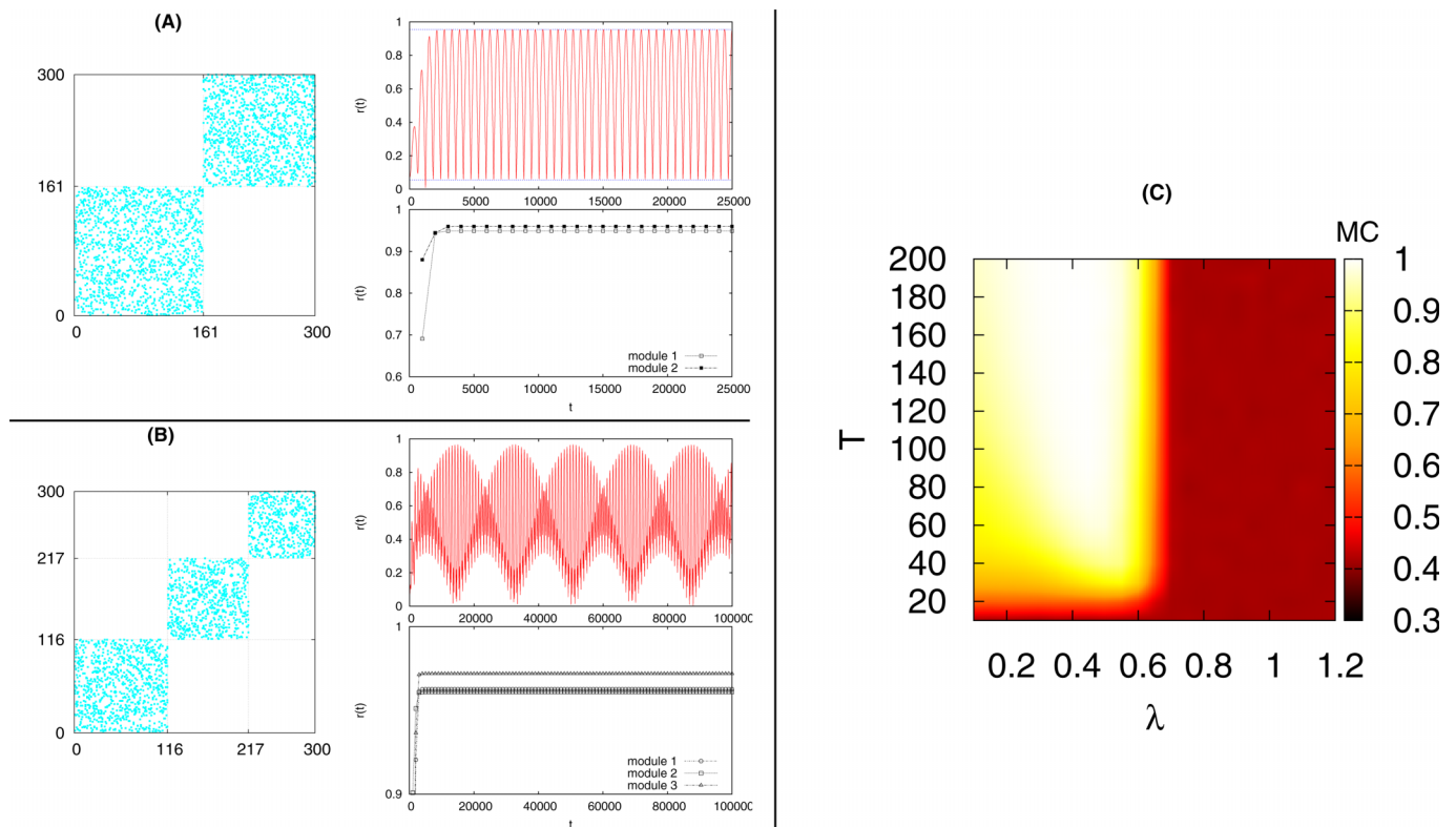
Figure 2 | Emergence of cluster structures in the partially ordered phase II. (A) For \lambda = 0.5 and T = 150 , the network splits into two components of similar size, while the global order parameter r oscillates harmonically in time. However, if r(t) is evaluated separately for the two clusters, a stationary value close to 1 is found in both cases. (B) For \lambda = 0.5 and T = 180 , the network splits into three components and the global order parameter displays a periodic behavior with three frequencies. Again, each component has an almost perfect degree of internal synchronization. The contour-plot in panel (C) reports the value of the modular cohesion MC as a function of \lambda and T . The large values of MC correspond to the high modular character of the network in phase II, and to the presence of a modular structure also in phase I.
