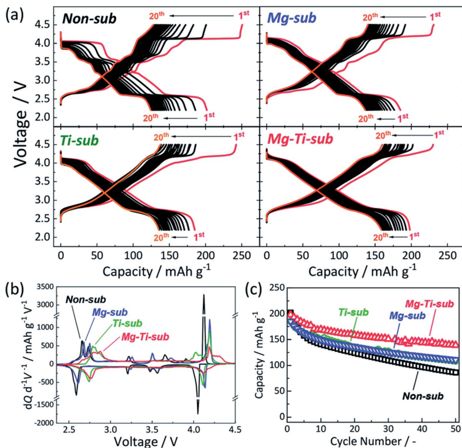
Fig. 10 (a) Galvanostatic charge–discharge plot, (b) dQ/dV plot, and (c) cyclic stability of Mg–Ti-sub, non-sub, Mg-sub and Ti-sub and electrodes in Na-ion cells. At 12 \text{ mA g}^{-1} current density galvanostatic charge–discharge experiments were conducted. (Adapted from ref. 60, copyright 2021 Royal Society of Chemistry).
