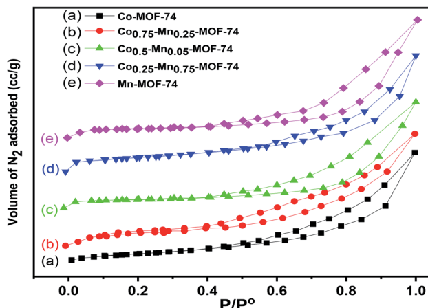
Fig. 3 Adsorption-desorption isotherms of nitrogen at 196 °C on monometallic and bimetallic MOFs.
