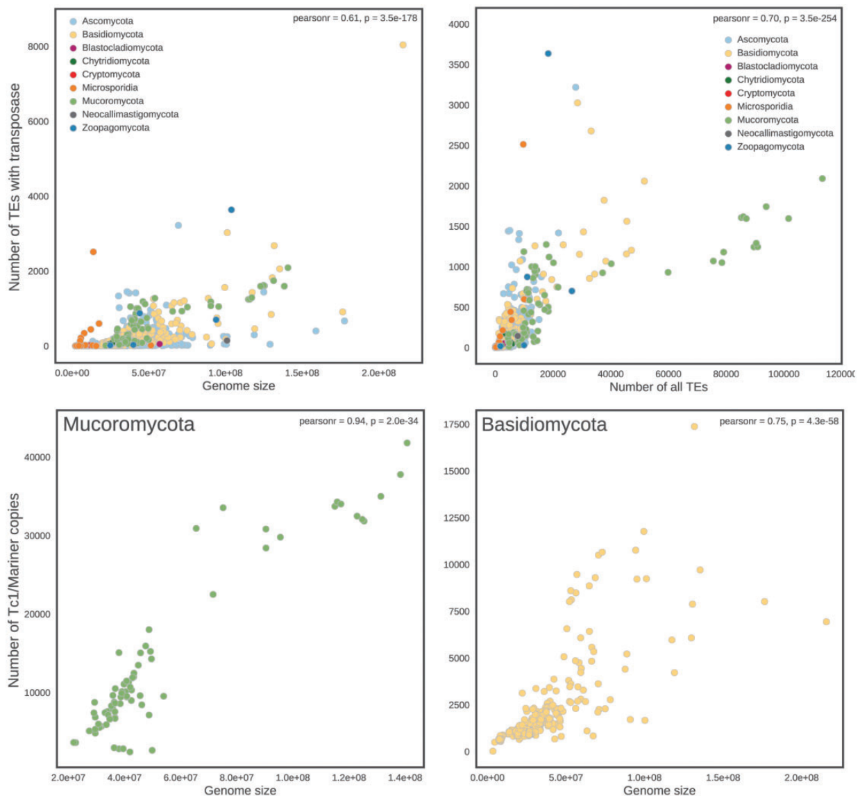
FIG. 3. —(A) Distribution of TE containing transposase versus genome size ( n = 1,726 ). (B) Correlation between the abundance of all and transposase-containing DNA TEs for each genome. Uromyces viciae-fabae outlier was not shown ( x = 91,391 , y = 8,039 ). Tc1/Mariner abundance in (C) Mucoromycota ( n = 74 ) and (D) Basidiomycota ( n = 314 ). The figure was prepared using Python in Jupyter (Kluyver et al. 2016).
