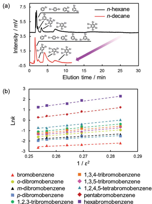
Fig. 6 Chromatograms of the mixture of brominated benzenes with the C70-coated column (a) and \text{Ln} k against 1/\epsilon^2 in each NA mobile phase (b). Conditions: column, C70-coated (Type-1, 25.5 cm \times 100 \mu m i.d.); flow rate; 2.0 \mu L \text{min}^{-1} ; mobile phase, n -hexane, n -heptane, n -octane, n -nonane, n -decane; temperature, 25 ^\circ\text{C} ; detection, UV 228 nm.
