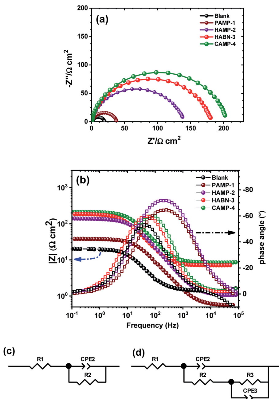
Fig. 3 (a) Nyquist diagrams for mild steel in 1 M HCl in the absence and in the presence of the various inhibitors ( 10^{-4} M) at 298 K. (b) Bode diagrams. Equivalent circuits used to fit the experimental data: (c) without inhibitor (d) in the presence of inhibitors.
