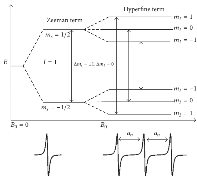
FIGURE 3: Energy level diagram of a nitroxide spin label in the presence of a magnetic field B_0 . The lower panel shows the corresponding EPR spectra in the absence and presence of a ^{14}\text{N} ( I = 1 ) hyperfine interaction.
