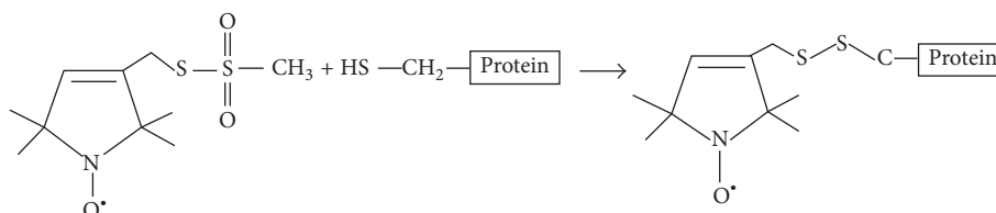
FIGURE 2: Structure of MTSL (methanethiosulfonate spin label) and the resulting side-chain produced by reaction with a cysteine residue on a protein.
