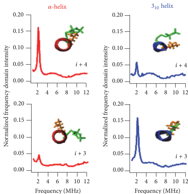
FIGURE 5: Three-pulse ESEEM FT data of ^2\text{H} -labeled \text{d}_{10} Leu4 LRL8 peptide in TFE ( \alpha -helix) and DPPC liposomes ( 3_{10} -helix) for i + 3 and i + 4 samples (adapted from [52] with permission).
