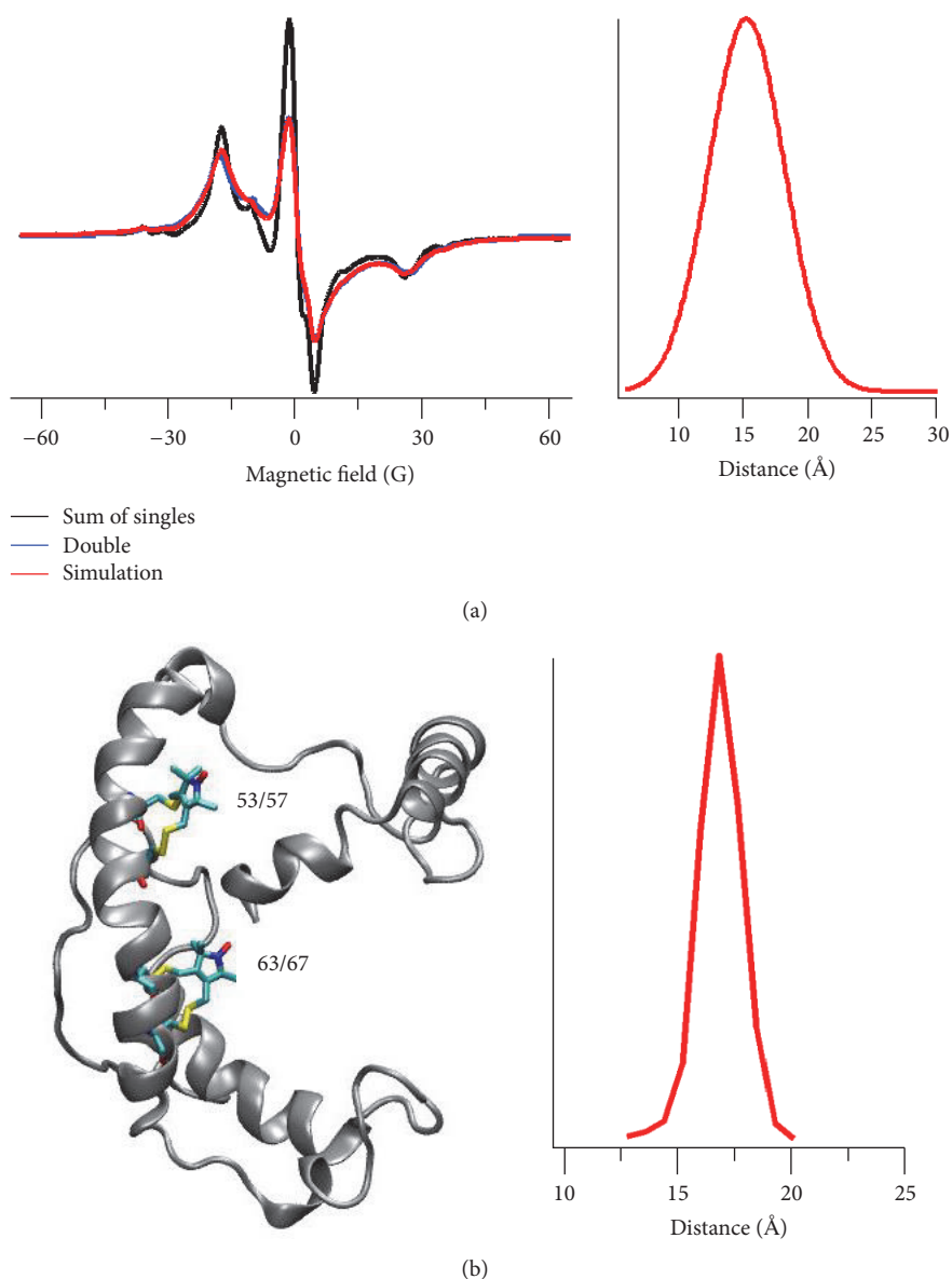
FIGURE 6: CW dipolar broadening EPR study of KCNE1. (a) CW dipolar broadening EPR spectra of KCNE1 bearing BSLs at sites 53/57 and 63/67 in POPC/POPG liposomes (left panel) and the corresponding distance distribution (right panel) obtained from data analysis by using the Short Distances LabVIEW program. (b) Cartoon representation of KCNE1 bearing two BSLs at sites 53/57 and 63/67 (left panel) and the corresponding distance distribution obtained from 20 ns molecular dynamics trajectory data analysis (right panel) (adapted from [53] with permission).
