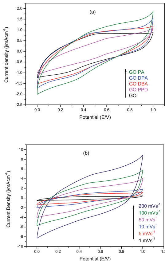
Fig. 11 Cyclic voltammograms in 1.0 \text{ M H}_2\text{SO}_4 of (a) amine-functionalized GOs at 10 \text{ mV s}^{-1} and (b) GO-PA at different scan rates.
