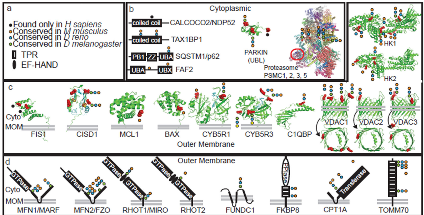
Figure 4. Structural anatomy and conservation of PARKIN-dependent diGLY sites Structures or domain schematics are shown for Class 1 depolarization and PARKIN-dependent diGLY sites (PDB codes, Table S5). Color-coded circles ( a ) indicate the conservation of Lys at the homologous position in M. musculus , D. rerio , and D. melanogaster (Table S5). For structures, regulated sites are shown in red space-filled models. b , Cytoplasmic proteins. RPN10, red circle. c , MOM proteins with structures. d , MOM proteins without structures.
