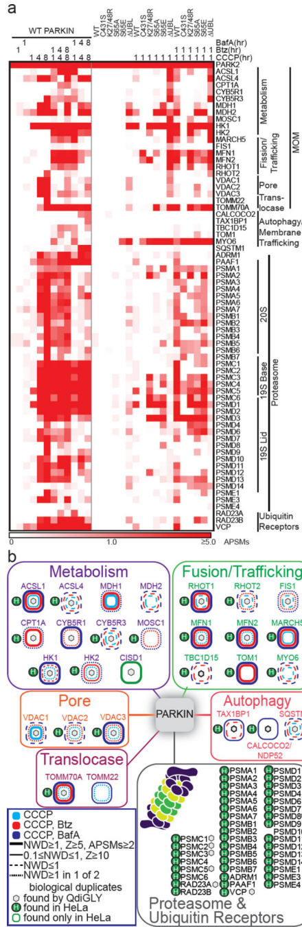
Figure 3. PARKIN associates with mitochondrial proteins and the proteasome in response to depolarization
