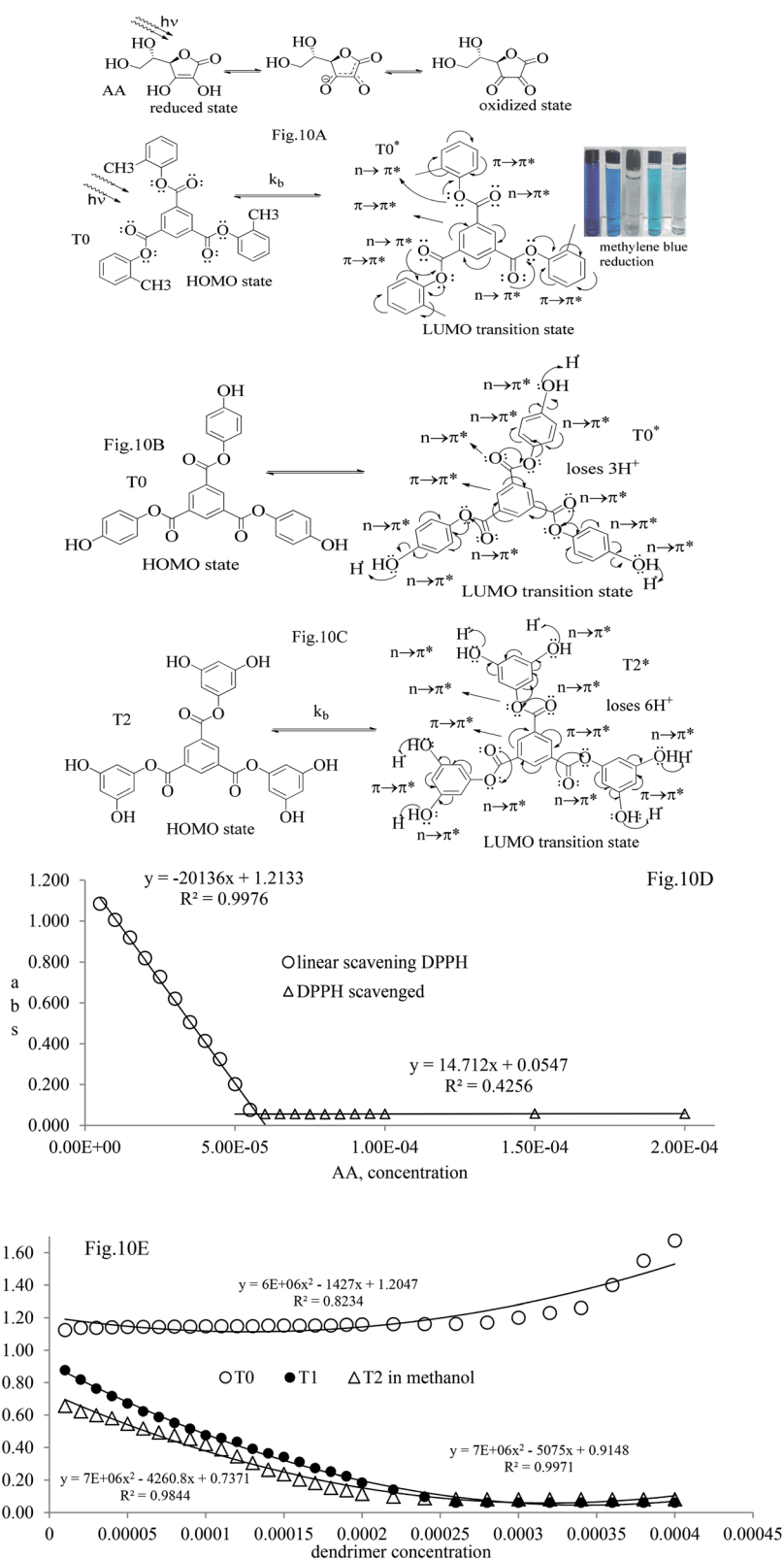
Fig. 10 (A–C) Optical activities from the HOMO to LUMO to scavenge DPPH radicals. (D) Abs vs. AA composition with 1 st order scavenging of DPPH free radicals. (E) Abs vs. dendrimer composition to scavenge DPPH free radicals.
