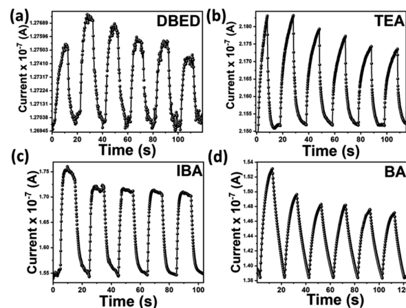
Fig. 8 The transient I-t (ON/OFF) curves of the devices of (a) DBED, (b) TEA, (c) IBA, and (d) BA perovskite-based photodetectors.
