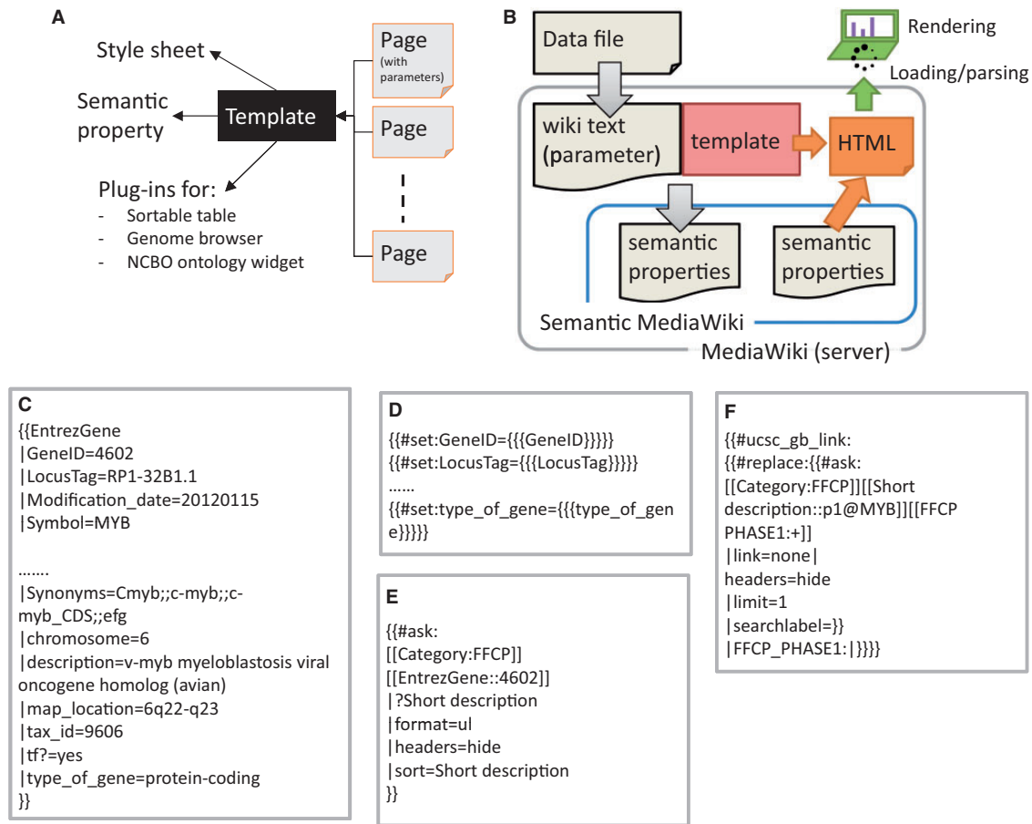
Figure 2. Implementation scheme of data model with SMW template. (A) Template dependencies. Each page in SSTAR use one or more template from SMW, the template points to different style sheets, calls semantic property and SSTAR plug-ins to deliver particular function. (B) Data flow from depositing the data file in MediaWiki server to render the page into the client. (C) Code snippet showing template call (EntrezGene) with the semantic properties to generate the page with EntrezGene:4602 http://fantom.gsc.riken.jp/5/ssstar/EntrezGene:4602 . (D) Statements in the 'EntrezGene' template to store template parameters as semantic properties. The statements will add the semantic properties 'GeneID', 'LocusTag' and 'type_of_gene'. (E) An example of inline semantic query, retrieving the association between two categories (gene and CAGE peaks) and show the result in an unnumbered list. (F) An example of the inline semantic query modified to call SSTAR ucsc_gb_link function to provide the genomic view of the FFCP in UCSC genome browser.
