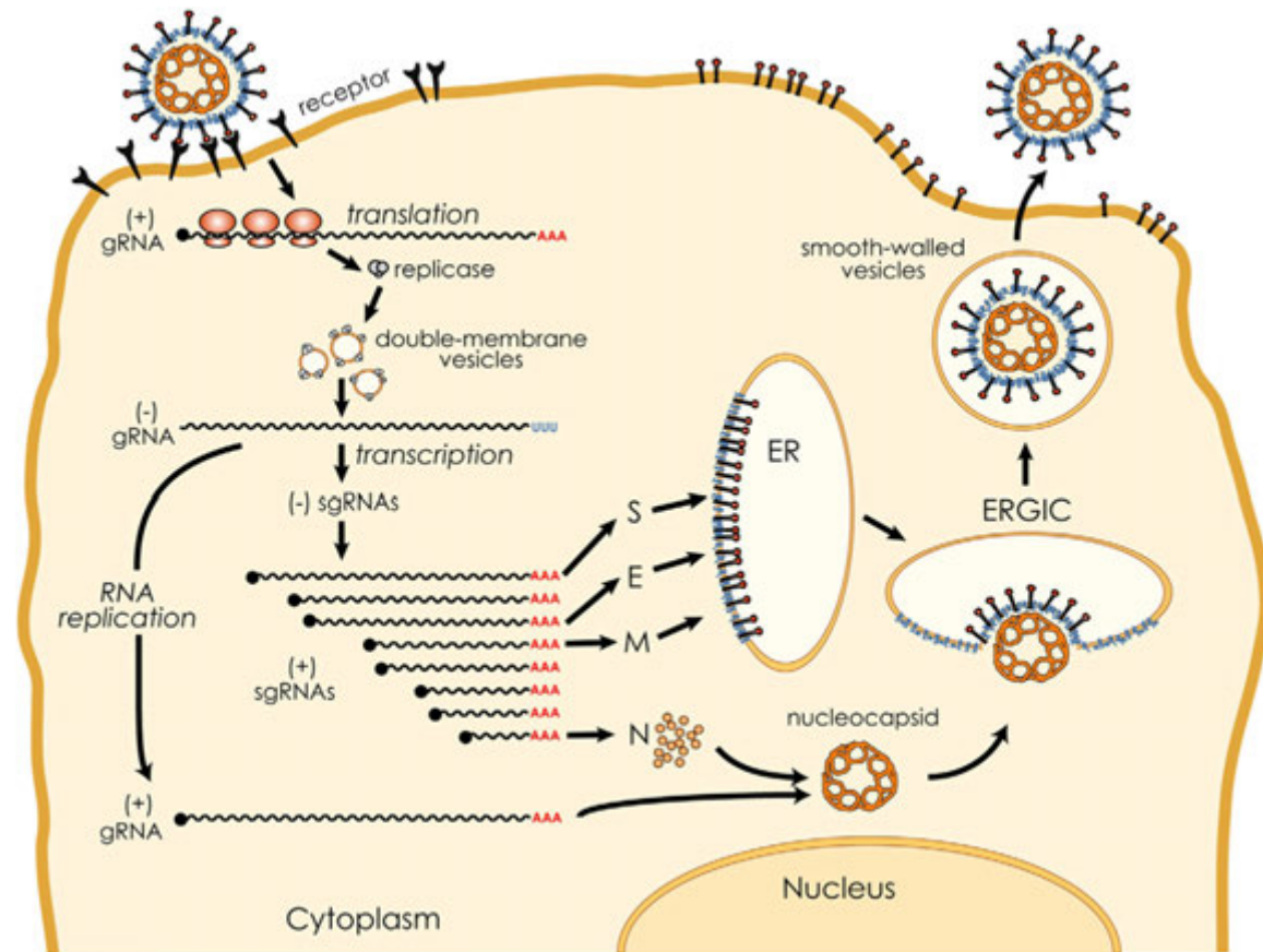
Fig. 4 Replication cycle of CoVs. The spike glycoprotein on the virus particle interacts with host cell receptors to mediate fusion of the virus and host cell membranes and release of the positive-strand RNA genome into the cytoplasm. The 5'-proximal open reading frames (ORF1a and ORF1b) are translated from the gRNA to generate the replicase polyprotein. The replicase polyprotein is processed by viral proteases into 16 nonstructural proteins which assemble with membranes to generate double-membrane vesicles (DMVs) where RNA synthesis takes place. A nested set of 3' co-terminal subgenomic (sg) RNAs is generated by a discontinuous transcription process. The sgRNAs are translated to generate the viral structural and accessory proteins. Viral gRNA is replicated and associates with nucleocapsid protein and viral structural proteins in the endoplasmic reticulum-Golgi intermediate compartment (ERGIC), where virus particles bud into vesicles before transport and release from the cell. Reprinted from Masters PS (2006) The molecular biology of coronaviruses. Advances in Virus Research 66: 193–292, with permission from Elsevier.
