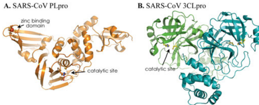
Fig. 6 CoV proteases are targets for antiviral drug development; X-ray structures of the two SARS-CoV protease domains encoded in the replicase polyprotein. (a) The SARS-CoV papain-like protease (PL pro ) with catalytic triad cysteine, histidine, and aspartic acid residues, and zinc-binding domain indicated. (b) The 3C-like protease (3CL pro , also termed main protease, M pro ) dimer with catalytic cysteine and histidine residues indicated.
