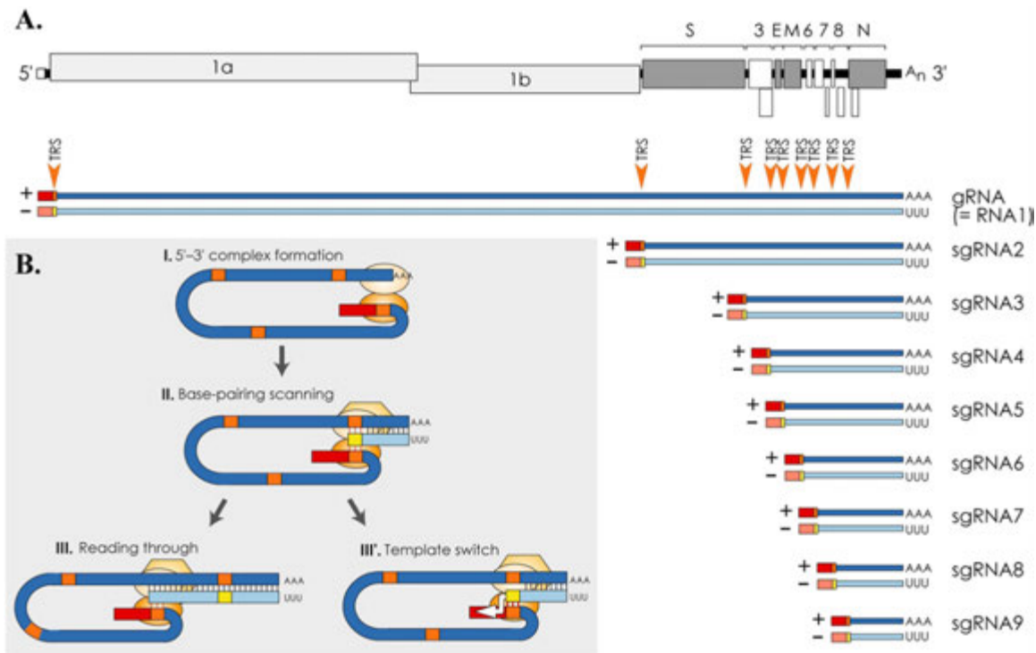
Fig. 5 Model of SARS-CoV gRNA and sgRNAs, and a working model of discontinuous transcription. (a) Diagram of gRNA and the nested set of sgRNAs of SARS-CoV. The 5' leader sequence, the transcriptional regulatory sequences (TRSs), and the positive- and negative-sense sgRNAs are indicated. (b) A working model of CoV discontinuous transcription. I. 5'–3' complex formation. Binding of viral and cellular proteins to the 5' and 3' ends of the CoV gRNA is represented by ellipsoids. The leader sequence is indicated in red, the TRS sites are in orange. II. Base-pair scanning step. Minus-strand RNA (light blue) is synthesized from the positive-strand template by the viral transcription complex (hexagon). At the TRS site, base-pairing may occur between the template, the nascent negative-strand RNA, and the leader TRS sequence (dotted lines). III. The synthesis of negative-strand RNA can continue to make a longer sgRNA III, or a template switch can take place III' to generate a leader-containing subgenomic negative-strand RNA, which could then serve as the template for leader-containing positive-strand sgRNAs. Modified from Enjuanes L, Almazán F, Sola I, and Zunia S (2006) Biochemical aspects of coronavirus replication: A virus–host interaction. Annual Reviews in Microbiology 60: 211–230.
