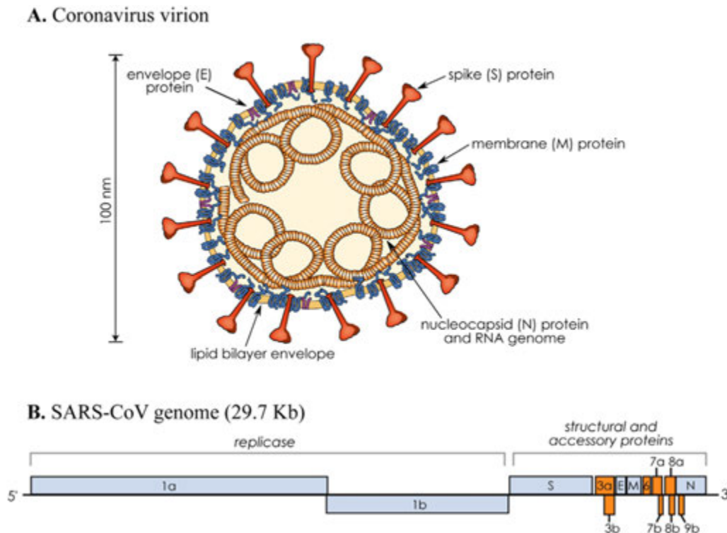
Fig. 2 CoV virion and the genome of SARS-CoV. (a) Schematic diagram of a CoV virion with the minimal set of four structural proteins required for efficient assembly of the infectious virus particles: S, spike glycoprotein; M, membrane glycoprotein; E, envelope protein; and N, nucleocapsid phosphoprotein which encapsidates the positive-strand RNA genome. (b) Schematic diagram of the gRNA of SARS-CoV. Translation of the first two open reading frames (ORF1a and ORF1b) generates the replicase polyprotein. ORFs encoding viral structural and accessory (orange) ORFs are indicated at the 3' end of the genome. (a) Reprinted from Masters PS (2006) The molecular biology of coronaviruses. Advances in Virus Research 66: 193–292, with permission from Elsevier.
