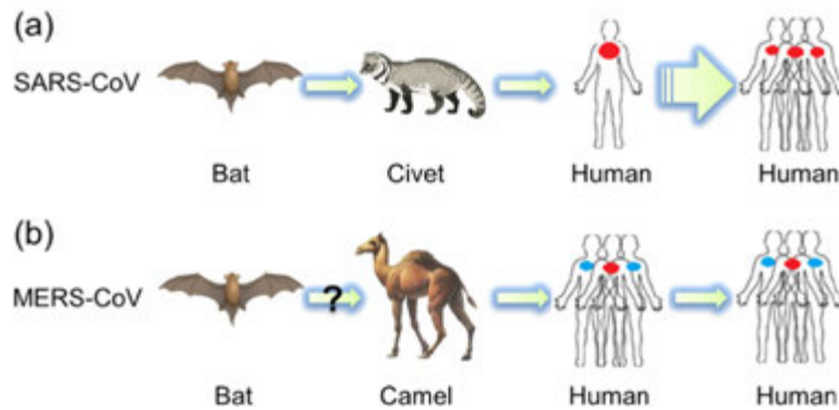
Fig. 1 Zoonotic transmission of emerging coronaviruses. (a) SARS-like coronaviruses are endemic in bats in Southern China. Virus transmission events may occur when animals are brought together in live animal markets. Replication of the virus in an intermediate host allows for the acquisition of adaptive mutations that allow for an expanded host range. SARS-CoV adapted to use the ACE-2 receptor in humans and can be spread by respiratory droplets. Infection with SARS-CoV generally results in symptomatic infection (red dots) characterized by fever and pneumonia. Super-spreader events (one person infecting many others) followed by global travel led to the pandemic of 2003. The quarantine of infected individuals and their contacts led to the cessation of the outbreak. (b) MERS-like viruses have been identified in bats and may be the progenitor of the virus now recognized to be endemic in camels in parts of the Middle East and Africa. MERS-CoV infection of camels seems to cause a respiratory disease with no significant mortality in young or adult camels. MERS-CoV infection in humans, proposed to be acquired from contact with camels or raw camel milk or meat, may cause pneumonia (red dot) or mild or asymptomatic illness (blue dot). Currently, there seems to be limited human-to-human transmission of MERS-CoV.
