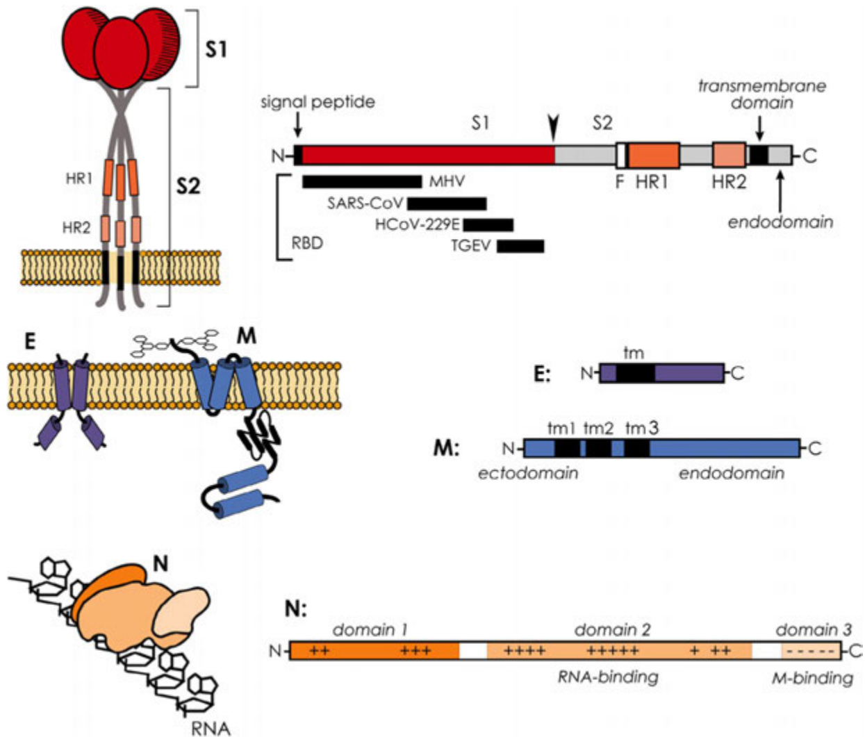
Fig. 3 Diagrammatic representation of the spike trimer assembled on membranes, with the S1 receptor binding domain (RBD) and S2 fusion domain indicated. The linear map of spike indicates the location of the RBDs for three CoVs, and the relative location of the heptad repeat domains 1 and 2 (HR1 and HR2) which mediate the conformational changes required to present the fusion peptide (F) to cellular membranes. The membrane (M), envelope (E), and nucleocapsid (N) proteins represented in association with membranes or viral RNA. The linear map of each protein highlights the transmembrane domains of M and E and the RNA-binding and M protein-binding domains of N. Domains 1 and 2 of N are rich in arginine and lysine (indicated by +). Reprinted from Masters PS (2006) The molecular biology of coronaviruses. Advances in Virus Research 66: 193–292, with permission from Elsevier.
