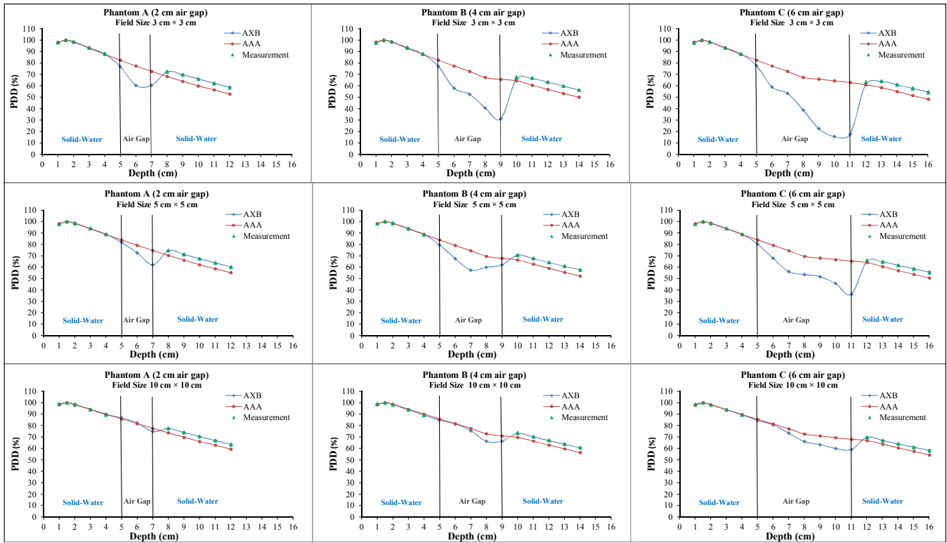
Figure 2: The measured PDD in the solid–water regions (upstream and downstream of air gap) and the calculated PDD curves by AAA and AXB in phantoms A (2-cm air gap), B (4-cm air gap), and C (6-cm air gap), (from left to right) for field sizes 3 × 3, 5 × 5, and 10 × 10 cm 2 (from top to bottom). (6 MV photon beam, 100 cm SSD, 100 MUs). Abbreviations: PDD = Percent Depth Dose, AAA = Anisotropic Analytical Algorithm, AXB = Acuros XB Algorithm, SSD = Source to Surface Distance, MUs = Monitor Units.
