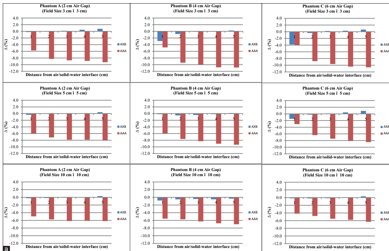
Figure 3: Comparisons between calculated and measured PDD at points between 1 and 5 cm distance from the air/solid–water interface in phantoms A (2-cm air gap), B (4-cm air gap), and C (6-cm air gap), (from left to right) for field sizes 3 \times 3 , 5 \times 5 , and 10 \times 10 cm 2 (from top to bottom). The \Delta (%) was calculated using Equation 1. (6 MV photon beam, 100 cm SSD, 100 MUs). Abbreviations: AAA = Anisotropic Analytical Algorithm, AXB = Acuros XB Algorithm, PDD = Percent Depth Dose, \Delta (%) = Dose Difference, SSD = Source to Surface Distance, MUs = Monitor Units.
