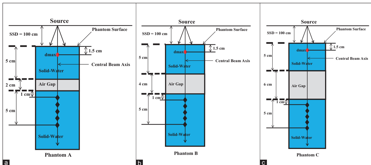
Figure 1: (a) schematic of the experimental setup for depth dose computations and measurements in phantom A (2-cm air gap), phantom, (b) (4-cm air gap), and phantom, (c) (6-cm air gap) (from left to right). Each layer (i.e., air gap and solid–water regions) in phantoms A, B, and C had rectangular area of 30 \times 30 \text{ cm}^2 . Central axis depth doses were compared in the first solid–water region (upstream of air gap) and second solid–water region (downstream of air gap). The common normalization point [i.e., depth of maximum dose ( d_{max} ) = 1.5 cm] that was used for dose computations and measurements is marked with red dot
