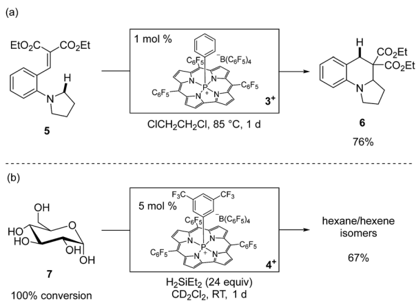
Scheme 3 (a) Reaction was performed on a 1.0 mmol scale. Isolated yield is reported. (b) Reaction was performed with 0.1 mmol of ^{13}\text{C}_6 -glucose. Quantitative ^{13}\text{C} NMR yields are reported. The ratio of products is 27 : 22 : 14 : 4 n -hexane : 3-methylpentane : 2-methylpentane : hexenes.
