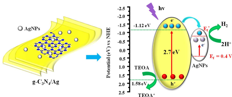
Fig. 8 Proposal mechanism for PH2P of g\text{-C}_3\text{N}_4/\text{Ag} .
