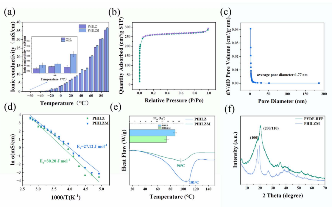
Fig. 3 (a) The ionic conductivities of PHILZM and PHILZ. (b) BET curves of ZIF-8. (c) Pore size distribution of ZIF-8. (d) The ionic conductivity–temperature curve of the gel polymer electrolytes fitted by the Arrhenius formula. (e) DSC of PHILZ and PHILZM. (f) XRD of PVDF-HFP and PHILZM.
