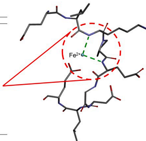
Fig. 4. The in silico interaction between peptides from whey isolate and fractionation and ferric iron ( Fe^{2+} ). Dates analyzed by AutoDock Vina®. Negative values mean spontaneous reaction. The most potent interaction between peptides and Fe^{2+} is in bold and is visualized using Discovery Studio 2016 Client®. The amino acids are presented in one letter nomenclature: A = Ala; C = Cys; D = Asp; E = Glu; F = Phe; G = Gly; H = His; I = Ile; K = Lys; L = Leu; M = Met; N = Asn; P = Pro; Q = Gln; R = Arg; S = Ser; T = Thr; V = Val; W = Trp; Y = Tyr. EFE: estimated free energy.
