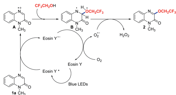
Scheme 5 Plausible mechanism.
