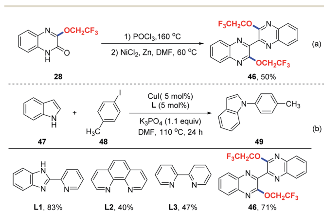
Scheme 3 Further chemistry.
