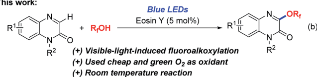
Scheme 1 The C3–H fluoroalkoxylation of quinoxalin-2(1 H )-ones.
