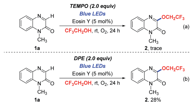
Scheme 4 Mechanism studies.
