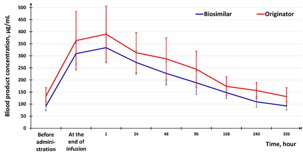
Fig. 2 Mean pharmacokinetic curves for the recorded eculizumab serum steady-state concentration in the extensive examination
