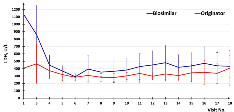
Fig. 4 Dynamics of lactate dehydrogenase activity during the study (95% CI for the mean)
