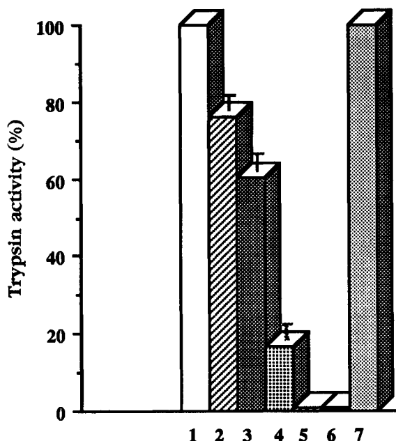
FIG. 1. Role of \alpha_2 -macroglobulin ( \alpha_2 -M) and soybean trypsin inhibitor (SBTI) on trypsin activity. Column 1, trypsin alone (14 \mu\text{g/ml} ); Columns 2, 3, 4 and 5, increased concentrations of \alpha_2 -M (200, 400, 600, 800 \mu\text{g/ml} ); Column 6, soybean trypsin inhibitor (15 \mu\text{g/ml} ); Column 7, \alpha_2 -M (800 \mu\text{g/ml} ) inactivated by methylammonium chloride (400 mM).
