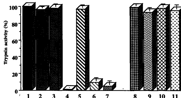
FIG. 3. Role of PMNL and MPO in \alpha_2 -M inactivation. Column 1, trypsin alone (14 \mu\text{g/ml} ); Column 2, trypsin + supernatant of activated PMNL; Column 3, trypsin + supernatant of non-activated PMNL; Column 4, trypsin + \alpha_2 -M (800 \mu\text{g/ml} ); Column 5, trypsin + \alpha_2 -M treated by supernatant of activated PMNL; Column 6, trypsin + \alpha_2 -M treated by supernatant of non-activated PMNL; Column 7, trypsin + \alpha_2 -M treated by activated PMNL preincubated with thiourea (10 -4 M); Column 8, trypsin + MPO (10 -7 M); Column 9, trypsin + HOCl (10 -7 M); Column 10, trypsin + \alpha_2 -M treated by MPO; Column 11, trypsin + \alpha_2 -M treated by HOCl (10 -7 M).
