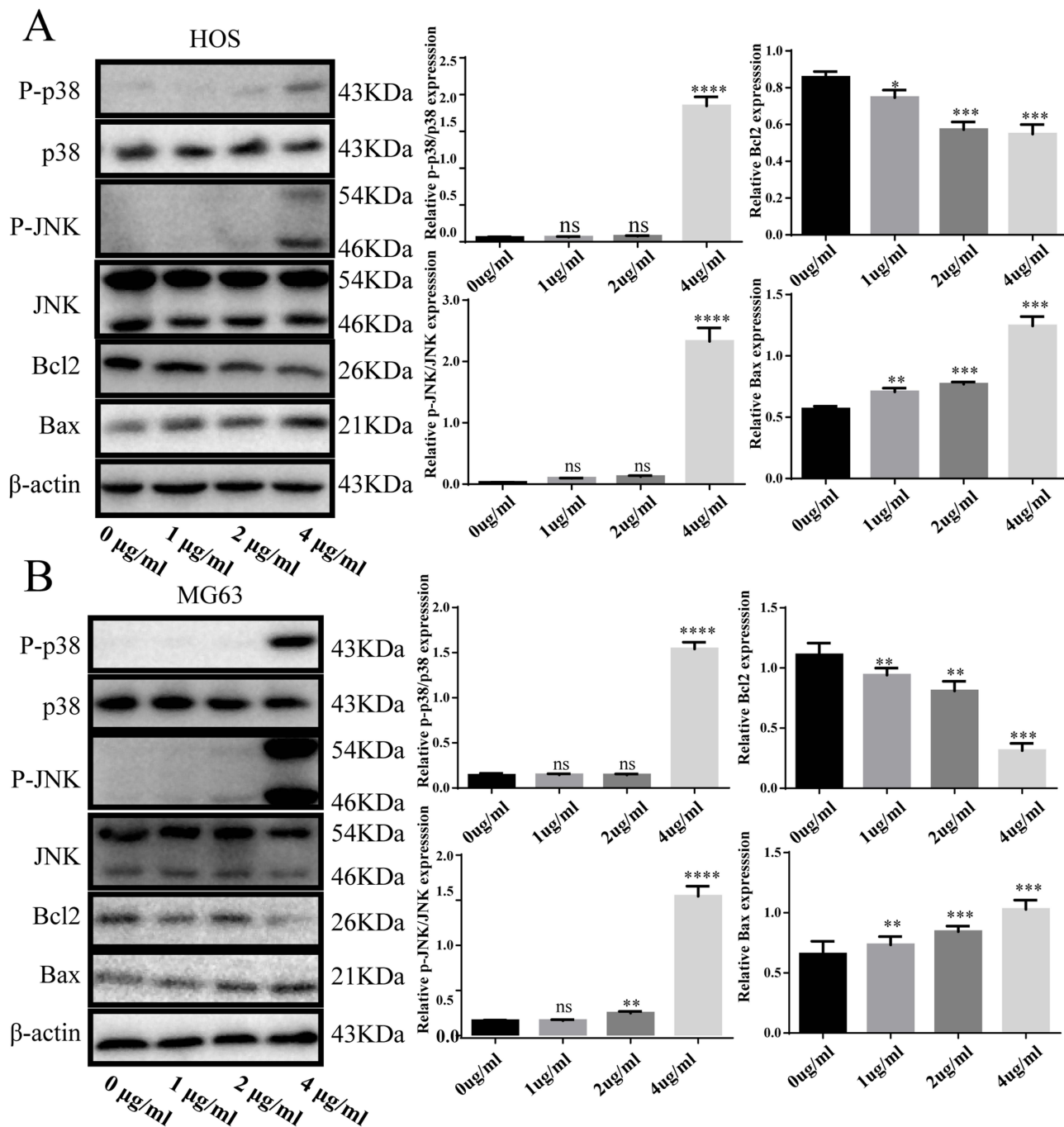
Figure 4 Activated p38/JNK signaling pathway is involved in DAELNs induced anti-osteosarcoma effects. (A) The expression of P-p38, P38, P-JNK, JNK, Bax and Bcl2 in HOS cells with administration of DAELNs by Western blotting. (B) The expression of P-p38, P38, P-JNK, JNK, Bax and Bcl2 in MG63 cells with administration of DAELNs by Western blotting. Data are shown as the mean \pm SEM. ns, no significance; * P < 0.05 , ** P < 0.01 , *** P < 0.001 , and **** P < 0.0001 .
