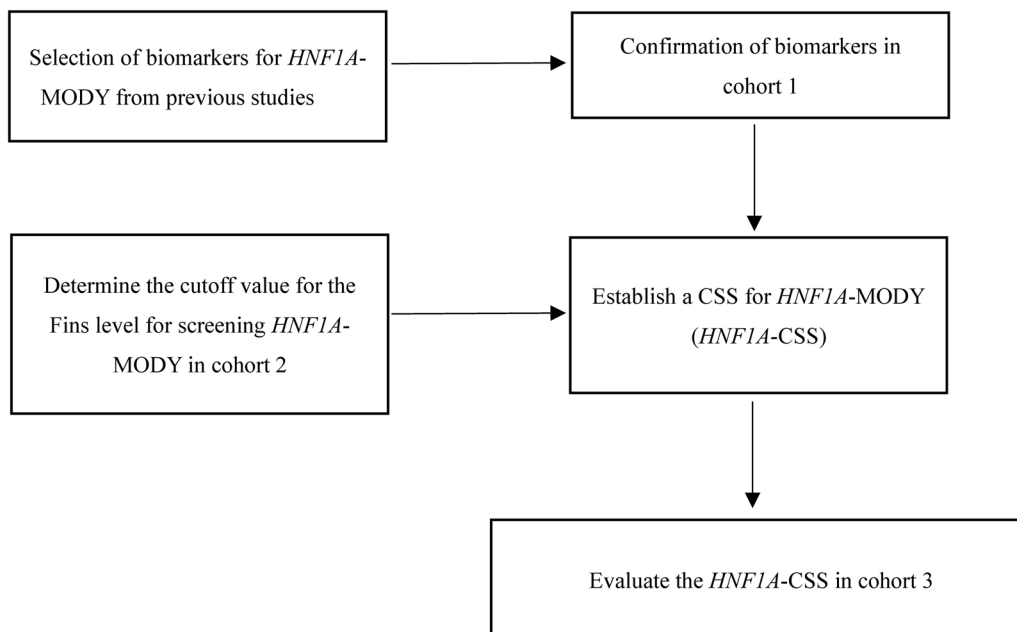
Figure 1 Flowchart showing the design of our study. CSS, clinical screening strategy; HNF1A , hepatocyte nuclear factor-1 alpha; MODY, maturity-onset diabetes of the young.
