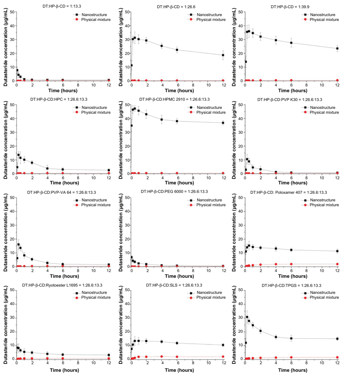
Figure 3 Supersaturated dissolution of a physical mixture and dutasteride-loaded HP- \beta -CD nanostructures with or without hydrophilic additives prepared using the supercritical antisolvent process.
