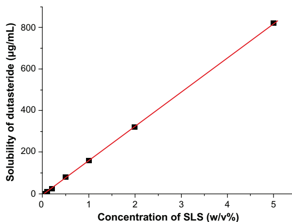
Figure 5 Effect of sodium lauryl sulfate concentration on the solubility of dutasteride.
