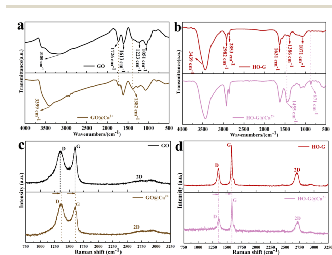
Fig. 1 FTIR spectra of (a) GO, \text{GO@Ca}^{2+} and (b) HO-G, \text{HO-G@Ca}^{2+} ; Raman spectra of (c) GO, \text{GO@Ca}^{2+} and (d) HO-G, \text{HO-G@Ca}^{2+} .
