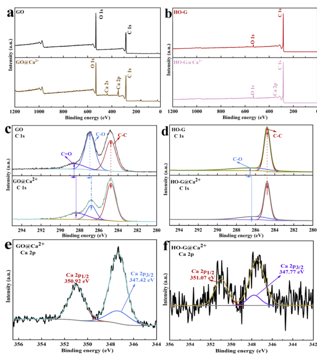
Fig. 2 XPS survey spectra of (a) GO, \text{GO@Ca}^{2+} and (b) HO-G, \text{HO-G@Ca}^{2+} ; high-resolution XPS C 1s spectra of (c) GO, \text{GO@Ca}^{2+} and (d) HO-G, \text{HO-G@Ca}^{2+} ; well-fitted XPS Ca 2p of (e) \text{GO@Ca}^{2+} and (f) \text{HO-G@Ca}^{2+} .
