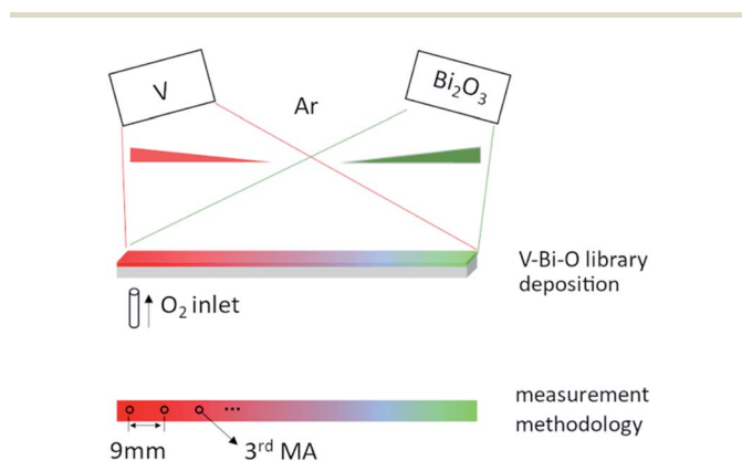
Fig. 1 Schematic (not to scale) of the co-sputter deposition of the \text{VO}_2\text{:Bi} library and its measurement areas (MAs) for characterizations (top view), the wedge shapes in the schematic denote the thickness gradients of sputtered material from each target in the library.
