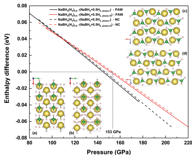
Fig. 10 Enthalpy difference between NaBH 4 + 0.5H 2 and NaBH 4 (H 2 ) 0.5 as a function of pressure. NC: Norm-Conserving method. PAW: Projector Augmented Wave method. View along the c axis of (a) the NaBH 4 Pnma structure and (b) the NaBH 4 (H 2 ) 0.5 P2 1 /c structure. View along the b axis of (c) the NaBH 4 Pnma structure and (d) the NaBH 4 (H 2 ) 0.5 P2 1 /c structure.
