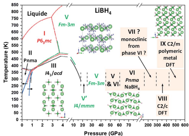
Fig. 9 Temperature vs. pressure phase diagram of LiBH 4 adapted and completed from past studies 33,40,43,46,47,51 (dotted lines: red – Pistorius; 41 black – Dmitriev et al. ; 43 blue – Sundqvist et al. ; 33 green – Yamawaki et al. 47 ). Green writing indicates a phase with disorder caused by tetrahedral reorientation. Red writing indicates a phase with disorder caused by tetrahedral rotation along one of its axes. Pressure range for the coexistence of phase V and VI is given for non-hydrostatic conditions; for helium pressure transmitting medium, this zone starts at 60 GPa and probably terminates near 80 GPa. Note that phase V' is considered as metastable 46 and that there is unconfirmed theoretical debate for structure of phase I. 73,74 Li, B and H atoms are respectively represented by light green, dark green and pink spheres. Phase VIII and IX are the phases from Yao & Klug for which the transition pressures were recalculated. Beige background indicates the new high pressure phase diagram proposed by this work.
