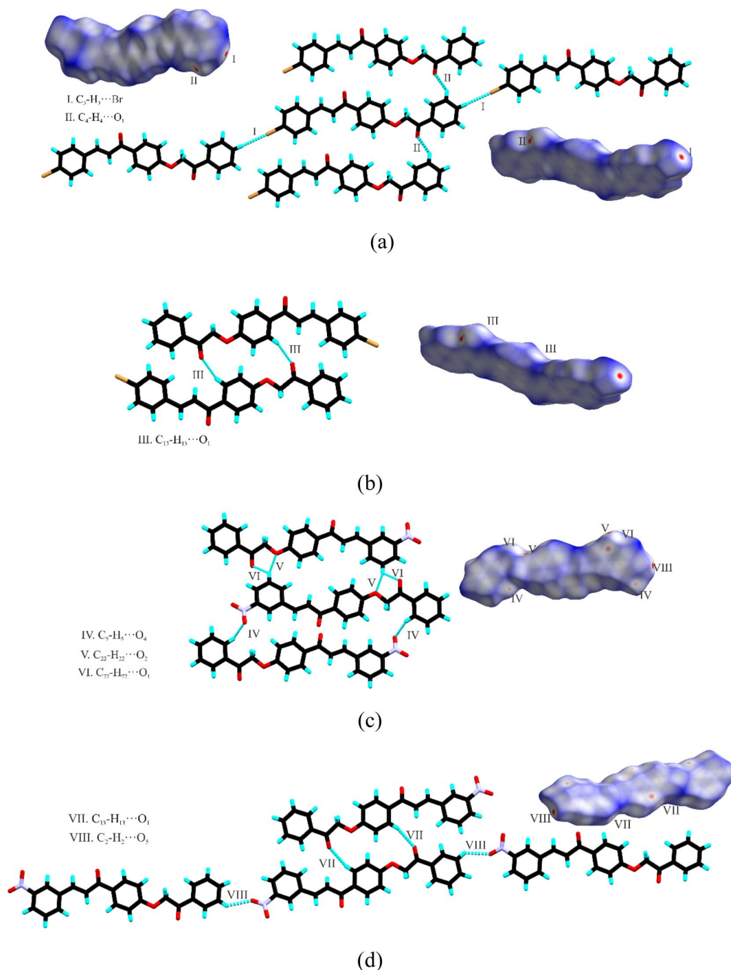
Fig. 2 The representation of interactions and HS d_{norm} showing the contacts for BCH (a) C_3-H_3...Br(i) C_4-H_4...O_1(ii) and (b) C_{13}-H_{13}...O_1(iii) . The NCH (c) C_5-H_5...O_4(iv) , C_{22}-H_{22}...O_2(v) and C_{22}-H_{22}...O_1(vi) and (d) C_{13}-H_{13}...O_1(vii) and C_2-H_2...O_5(viii) .
