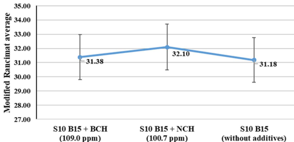
Fig. 5 The measurement uncertainty estimate of oxidation stability results from the modified Rancimat method.
