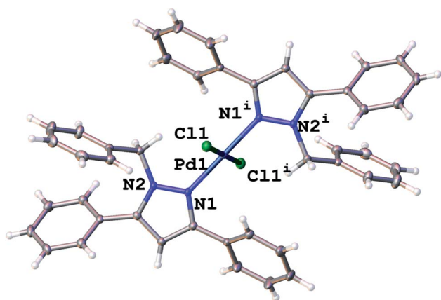
Fig. 1 Molecular structure of 7. Selected bond distance ( \text{\AA} ) and bond angles ( ^\circ ): Pd(1)–Cl(1) 2.2924(4), Pd(1)–N(1) 2.0135(15), N(2)–N(1) 1.363(2); N(1)–Pd(1)–Cl(1) 90.39(4)^\circ , N(1)–Pd(1)–Cl(1) 89.61(4)^\circ .
