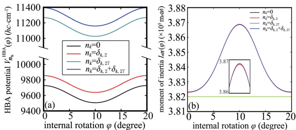
Fig. 3 (a) The potential V_{n_b}^{\text{HBA}}(\varphi) for the harmonic-bath averaged Hamiltonian in eqn (10) with given quantum numbers n_b for the normal modes perpendicular to the reaction path. (b) The effective moment of inertia I_{\text{eff}}(\varphi) for the internal rotation with given quantum numbers n_b . The green line indicates the zero-order moment of inertia I_0 . Four different cases of n_b are investigated in both (a) and (b).
