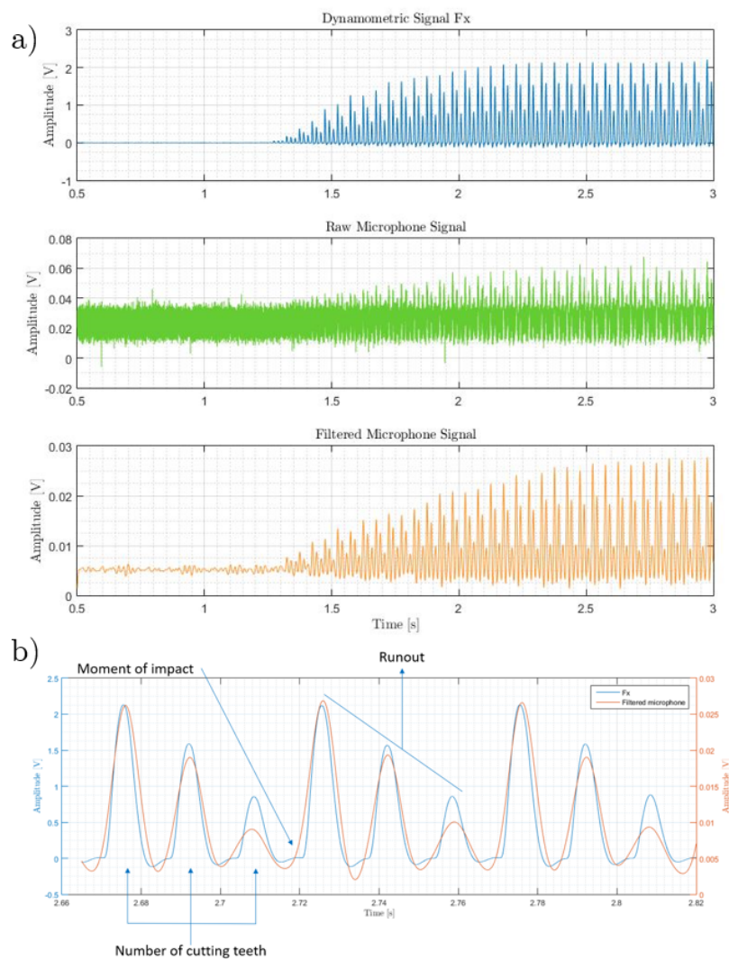
Figure 8. Experimental signals under analysis. (a) Cutting force signal (top), raw AE signal (middle), and filtered AE signal (bottom). (b) Zoomed section of the cutting force and filtered AE signals within the zone of uniform cut.
