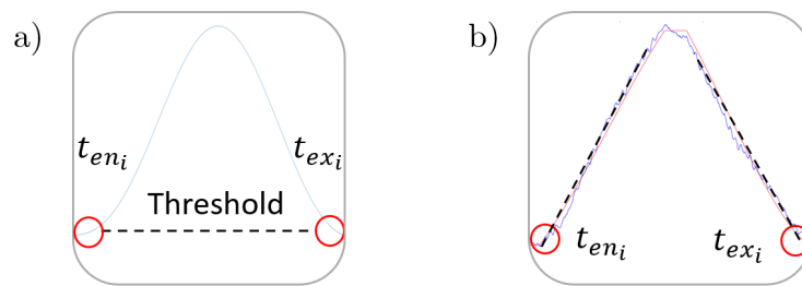
Figure 6. Time parameters measurement. (a) Threshold-based algorithm. (b) Slope-based algorithm.
