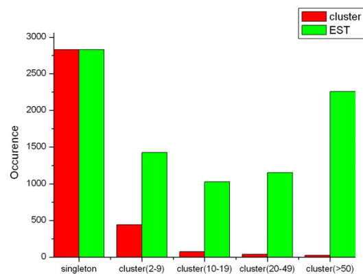
Figure 3 Prevalence distribution of the cluster size. The initial 8696 ESTs were grouped into 3416 clusters, consisting of 25 clusters (2257 of 8696 ESTs) that comprised of more than 50 ESTs each cluster, 39 clusters contained 20~49 ESTs (1153 of 8696 ESTs), 75 clusters contained 10~19 ESTs (1029 of 8696 ESTs), 445 clusters comprised 2~9 ESTs each cluster (1425 of 8696 ESTs), and 2832 unique sequence.
