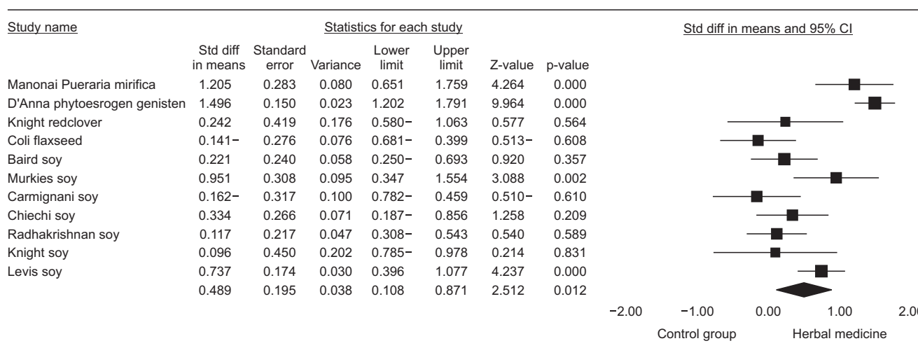
Fig. 2. Effects of herbal medicine on vaginal epithelial cells (%). Horizontal line: 95% confidence interval (CI), ■: point estimate, ◆: combined overall effect of treatment.
